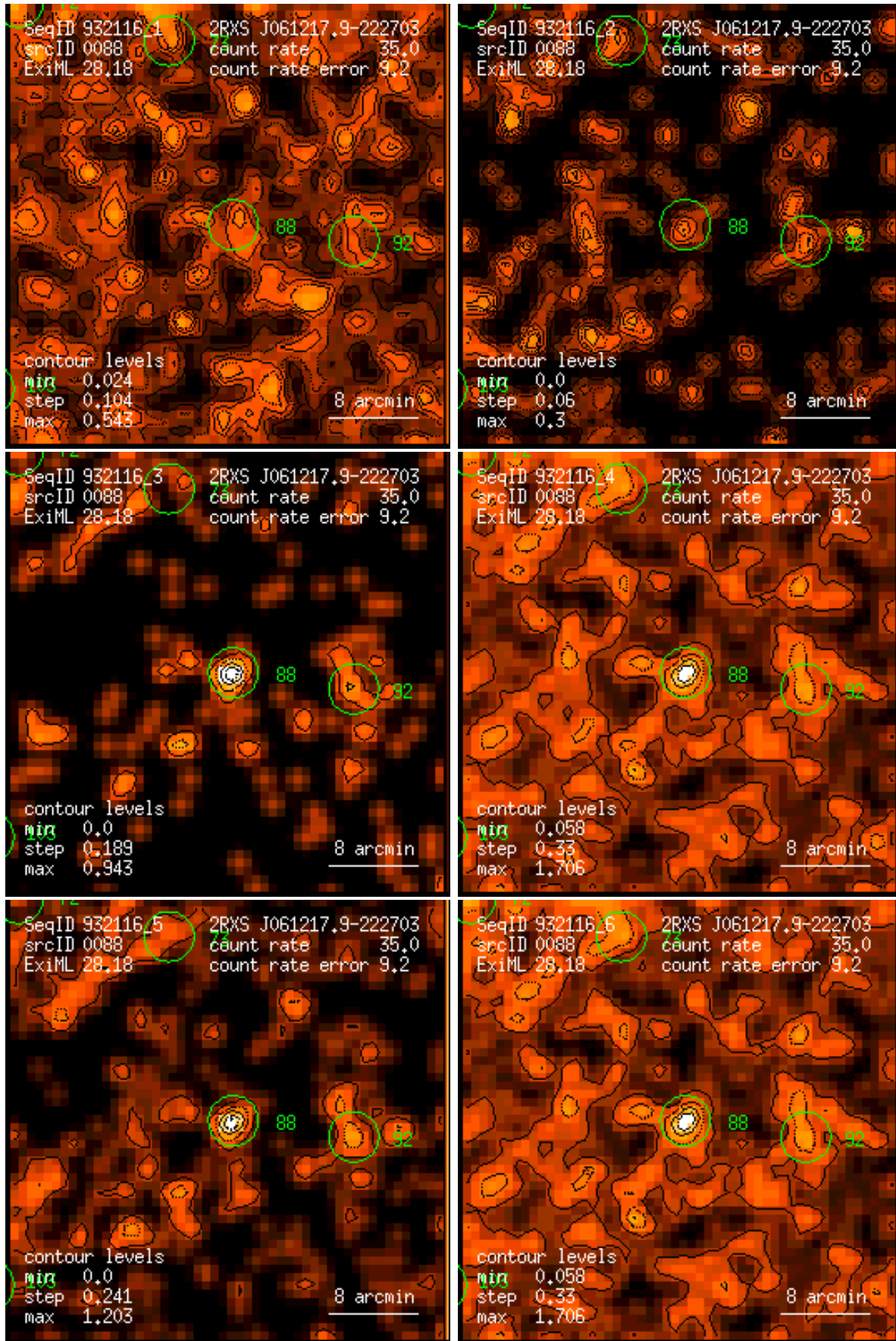
Figure 88: RASS 932116: detection 0088: band rate images, Gaussian filter: (1) PSPC channels 11 – 41, (2) 52 – 90, (3) 91 – 201, (4) 11 – 235, (5) 52 – 201, (6) 11 – 201. Broad band rates in counts/ks. Band rate contour levels in counts/ks/arcmin 2 .
