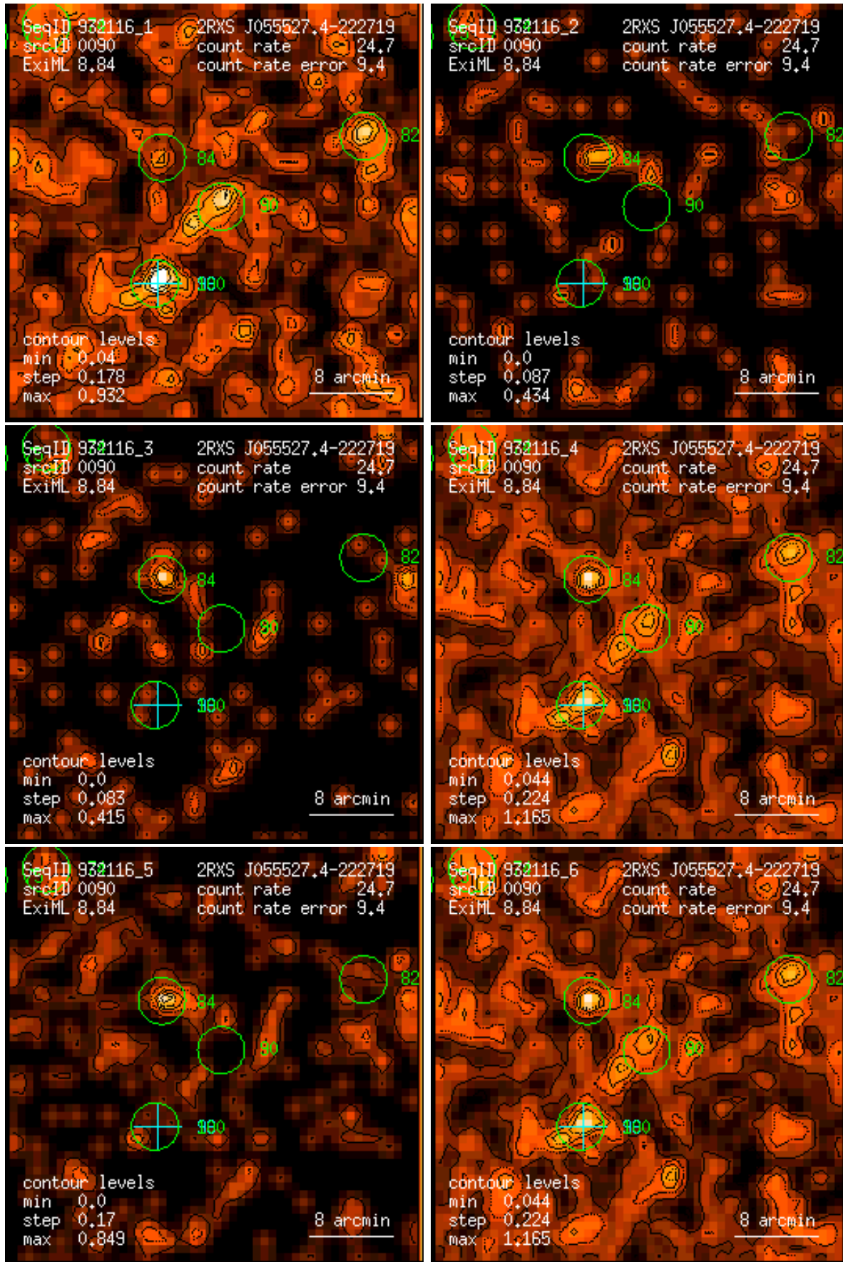
Figure 90: RASS 932116: detection 0090: band rate images, Gaussian filter: (1) PSPC channels 11 – 41, (2) 52 – 90, (3) 91 – 201, (4) 11 – 235, (5) 52 – 201, (6) 11 – 201. Broad band rates in counts/ks. Band rate contour levels in counts/ks/arcmin 2 .
