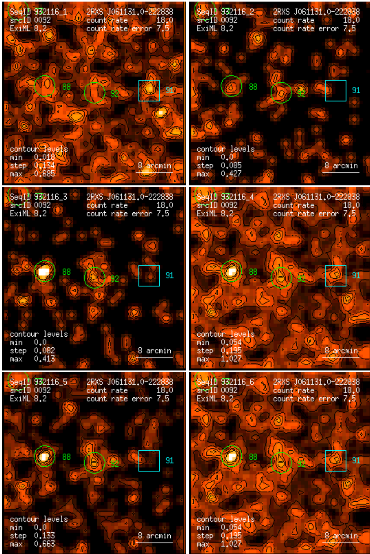
Figure 92: RASS 932116: detection 0092: band rate images, Gaussian filter: (1) PSPC channels 11 – 41, (2) 52 – 90, (3) 91 – 201, (4) 11 – 235, (5) 52 – 201, (6) 11 – 201. Broad band rates in counts/ks. Band rate contour levels in counts/ks/arcmin 2 .
