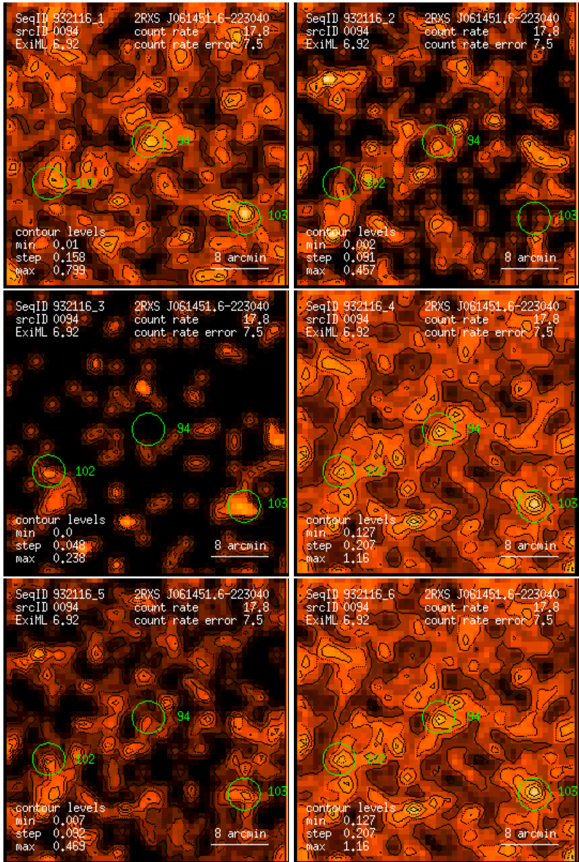
Figure 94: RASS 932116: detection 0094: band rate images, Gaussian filter: (1) PSPC channels 11 – 41, (2) 52 – 90, (3) 91 – 201, (4) 11 – 235, (5) 52 – 201, (6) 11 – 201. Broad band rates in counts/ks. Band rate contour levels in counts/ks/arcmin 2 .
