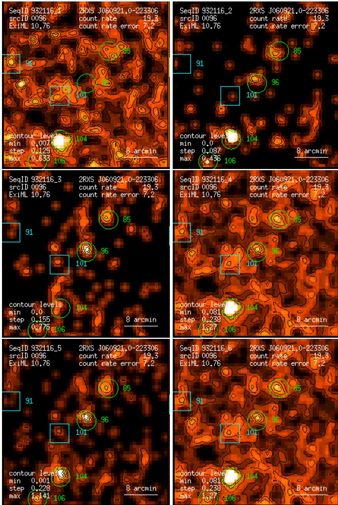
Figure 96: RASS 932116: detection 0096: band rate images, Gaussian filter: (1) PSPC channels 11 – 41, (2) 52 – 90, (3) 91 – 201, (4) 11 – 235, (5) 52 – 201, (6) 11 – 201. Broad band rates in counts/ks. Band rate contour levels in counts/ks/arcmin 2 .
