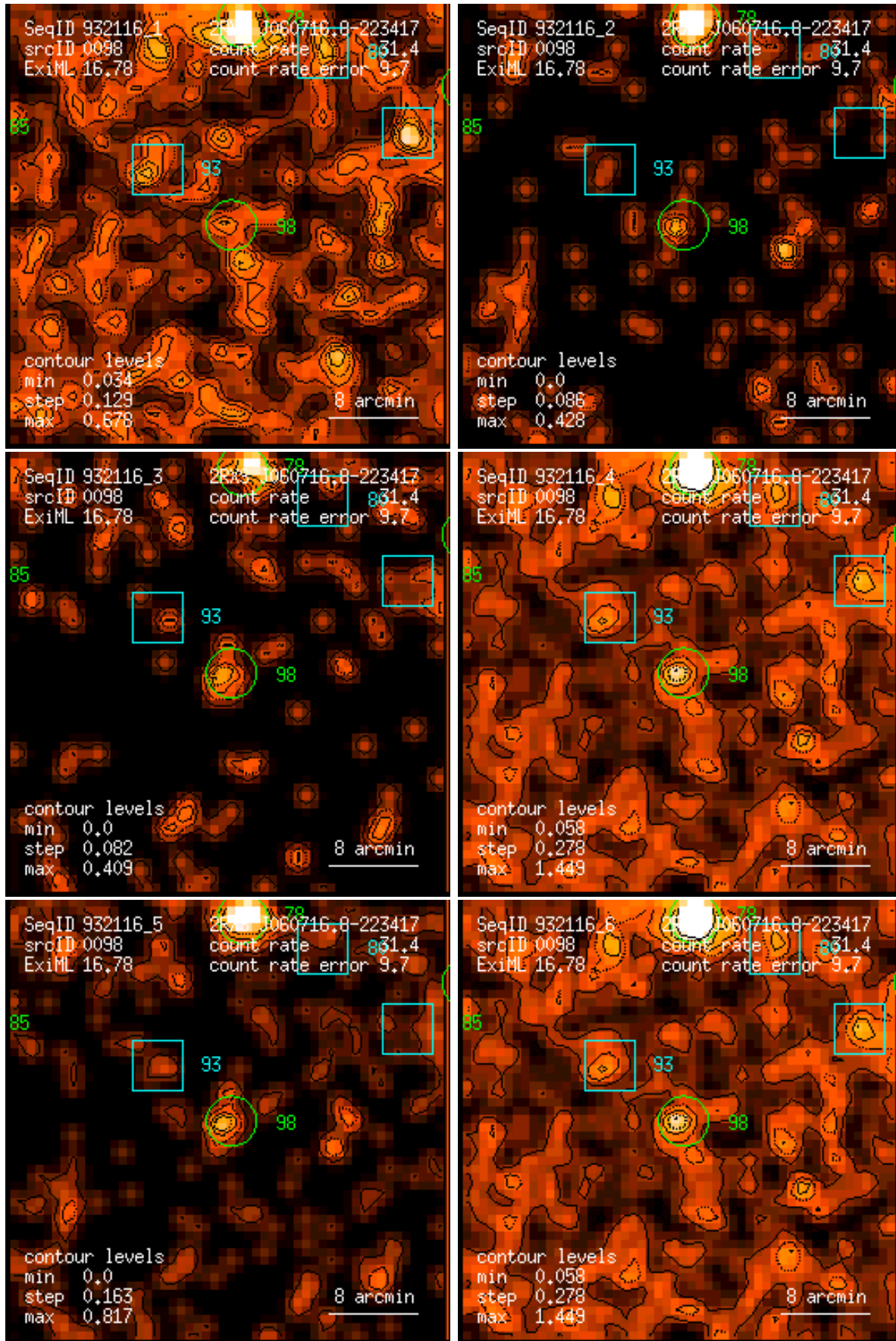
Figure 98: RASS 932116: detection 0098: band rate images, Gaussian filter: (1) PSPC channels 11 – 41, (2) 52 – 90, (3) 91 – 201, (4) 11 – 235, (5) 52 – 201, (6) 11 – 201. Broad band rates in counts/ks. Band rate contour levels in counts/ks/arcmin 2 .
