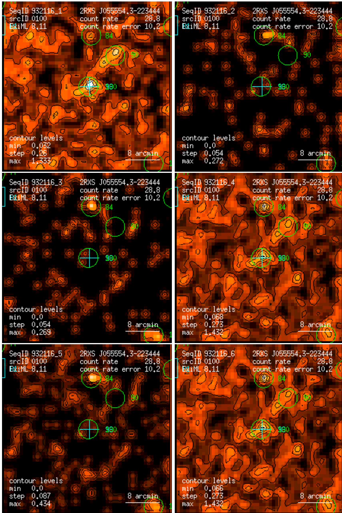
Figure 100: RASS 932116: detection 0100: band rate images, Gaussian filter: (1) PSPC channels 11 – 41, (2) 52 – 90, (3) 91 – 201, (4) 11 – 235, (5) 52 – 201, (6) 11 – 201. Broad band rates in counts/ks. Band rate contour levels in counts/ks/arcmin 2 .
