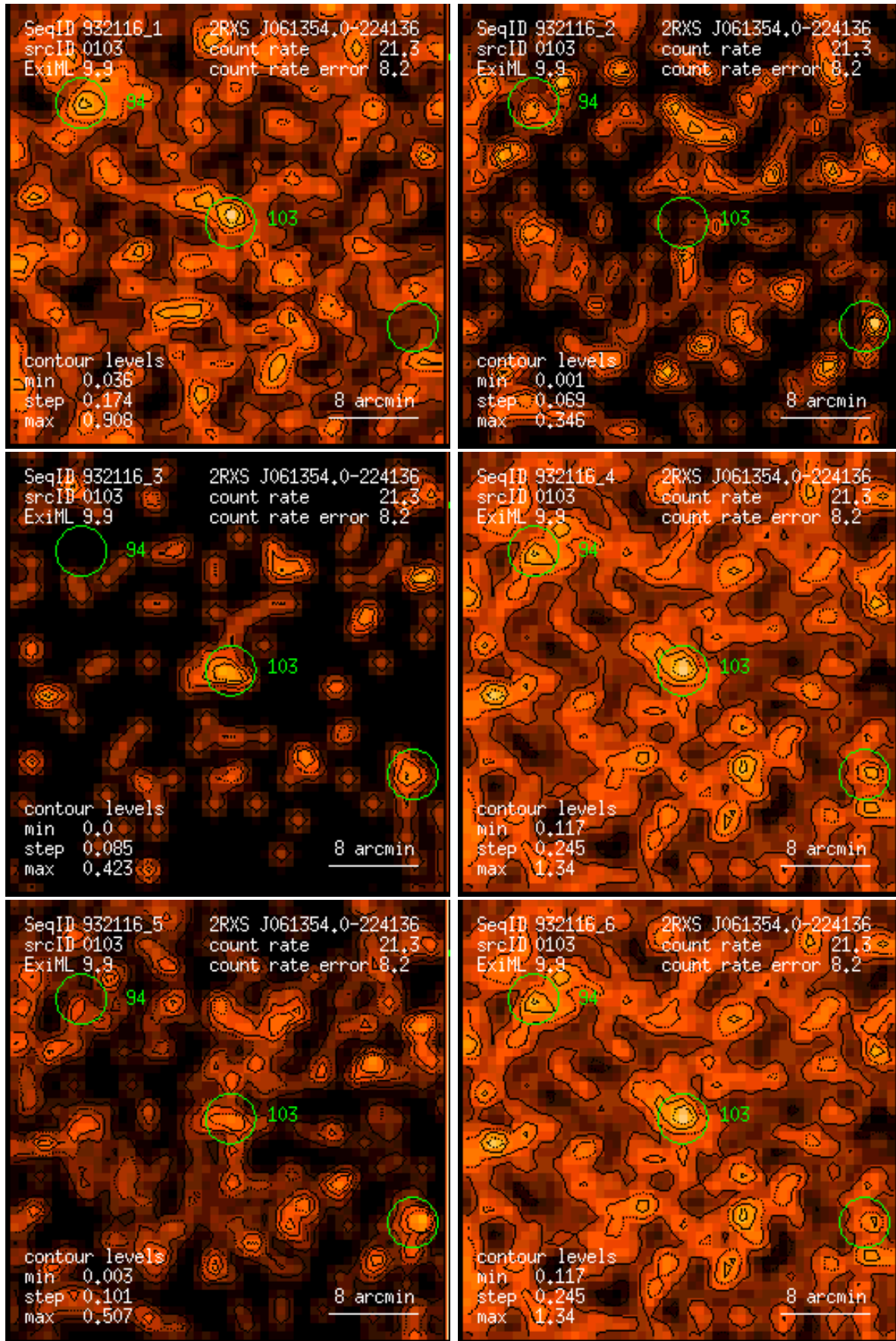
Figure 103: RASS 932116: detection 0103: band rate images, Gaussian filter: (1) PSPC channels 11 – 41, (2) 52 – 90, (3) 91 – 201, (4) 11 – 235, (5) 52 – 201, (6) 11 – 201. Broad band rates in counts/ks. Band rate contour levels in counts/ks/arcmin 2 .
