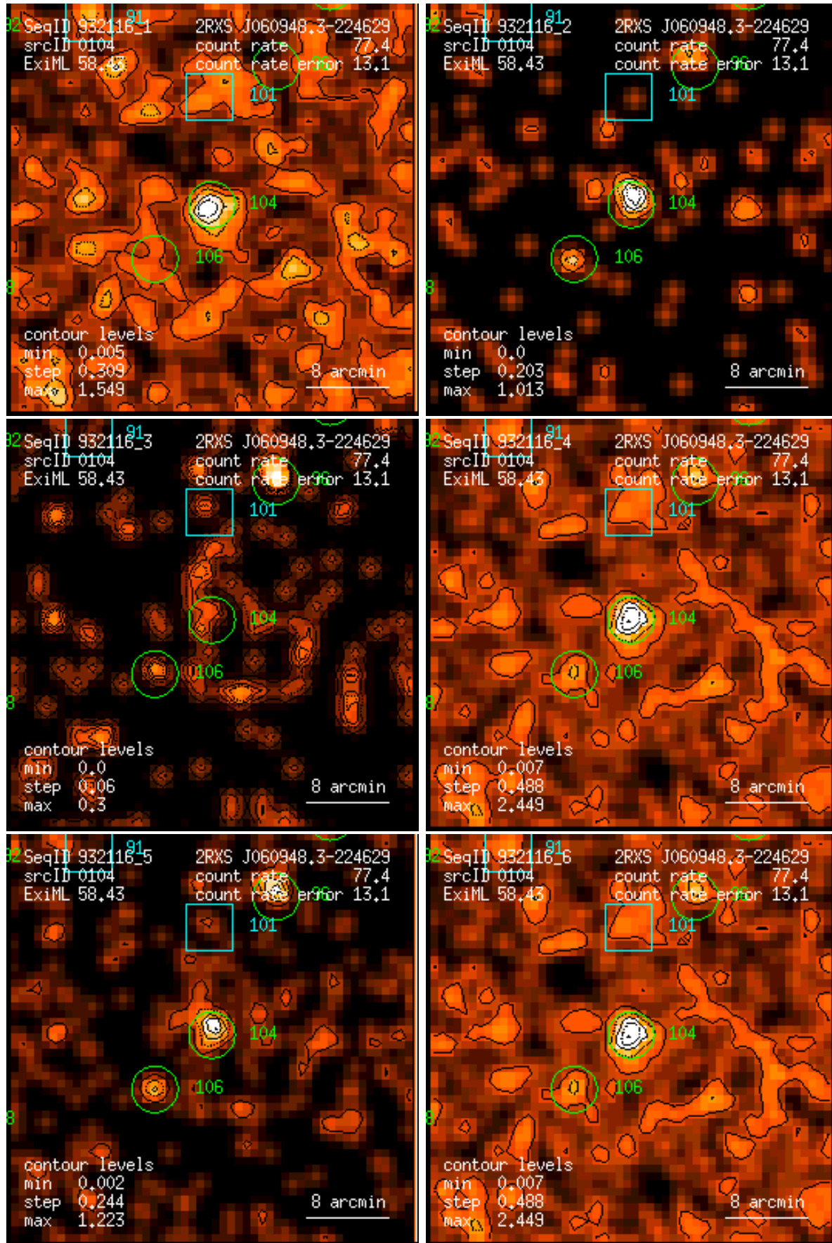
Figure 104: RASS 932116: detection 0104: band rate images, Gaussian filter: (1) PSPC channels 11 – 41, (2) 52 – 90, (3) 91 – 201, (4) 11 – 235, (5) 52 – 201, (6) 11 – 201. Broad band rates in counts/ks. Band rate contour levels in counts/ks/arcmin 2 .
