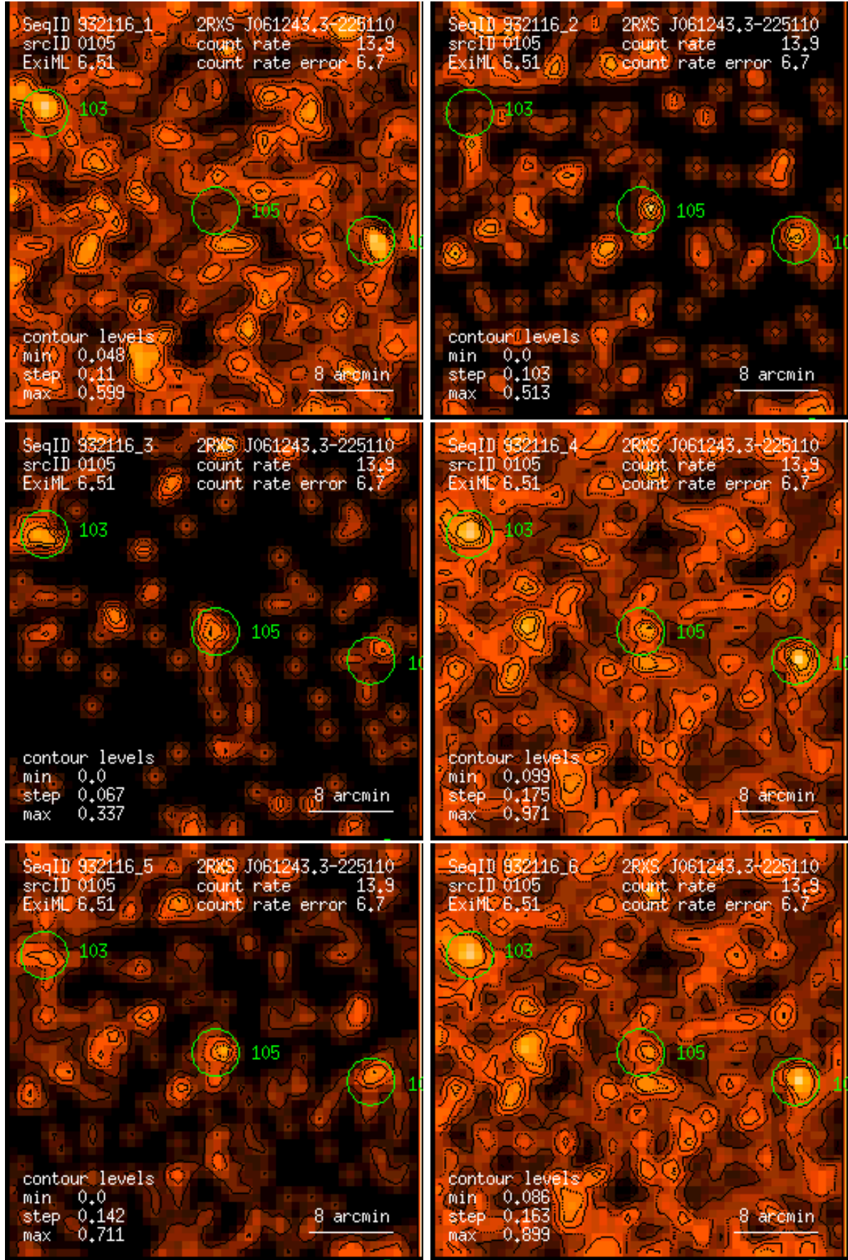
Figure 105: RASS 932116: detection 0105: band rate images, Gaussian filter: (1) PSPC channels 11 – 41, (2) 52 – 90, (3) 91 – 201, (4) 11 – 235, (5) 52 – 201, (6) 11 – 201. Broad band rates in counts/ks. Band rate contour levels in counts/ks/arcmin 2 .
