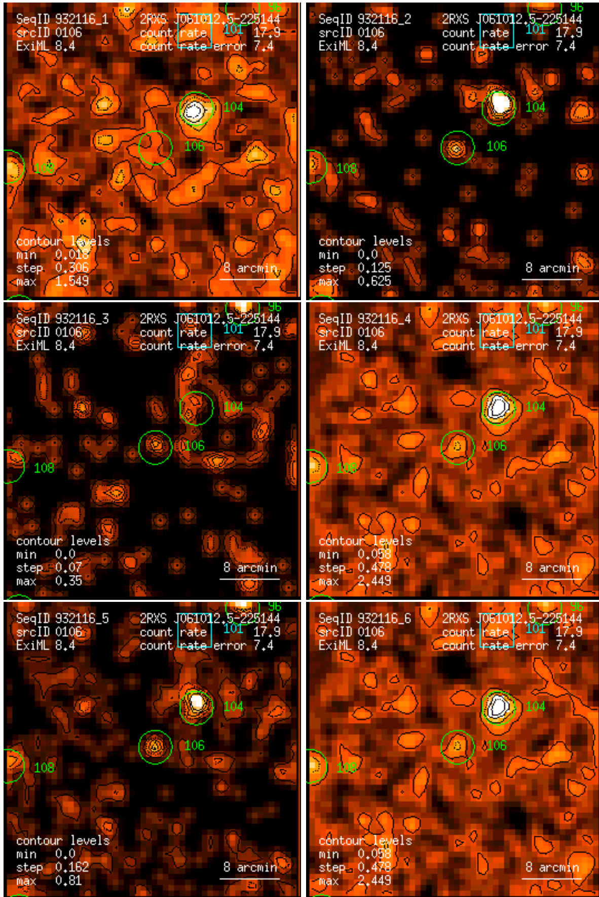
Figure 106: RASS 932116: detection 0106: band rate images, Gaussian filter: (1) PSPC channels 11 – 41, (2) 52 – 90, (3) 91 – 201, (4) 11 – 235, (5) 52 – 201, (6) 11 – 201. Broad band rates in counts/ks. Band rate contour levels in counts/ks/arcmin 2 .
