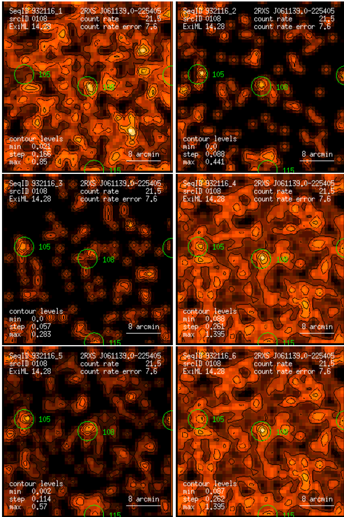
Figure 108: RASS 932116: detection 0108: band rate images, Gaussian filter: (1) PSPC channels 11 – 41, (2) 52 – 90, (3) 91 – 201, (4) 11 – 235, (5) 52 – 201, (6) 11 – 201. Broad band rates in counts/ks. Band rate contour levels in counts/ks/arcmin 2 .
