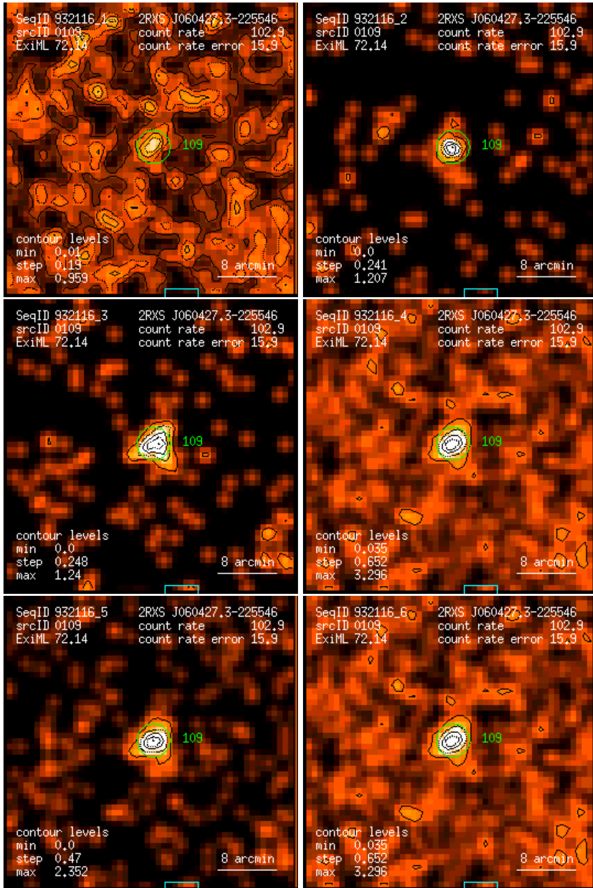
Figure 109: RASS 932116: detection 0109: band rate images, Gaussian filter: (1) PSPC channels 11 – 41, (2) 52 – 90, (3) 91 – 201, (4) 11 – 235, (5) 52 – 201, (6) 11 – 201. Broad band rates in counts/ks. Band rate contour levels in counts/ks/arcmin 2 .
