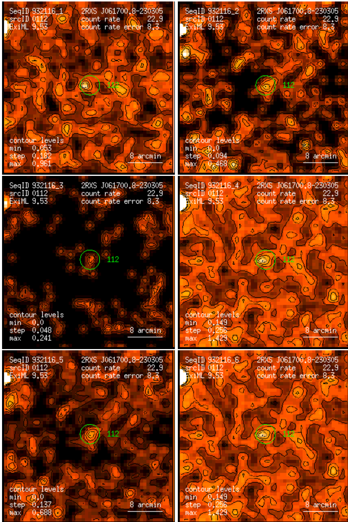
Figure 112: RASS 932116: detection 0112: band rate images, Gaussian filter: (1) PSPC channels 11 – 41, (2) 52 – 90, (3) 91 – 201, (4) 11 – 235, (5) 52 – 201, (6) 11 – 201. Broad band rates in counts/ks. Band rate contour levels in counts/ks/arcmin 2 .
