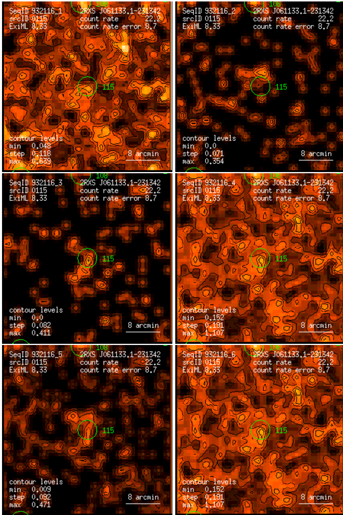
Figure 115: RASS 932116: detection 0115: band rate images, Gaussian filter: (1) PSPC channels 11 – 41, (2) 52 – 90, (3) 91 – 201, (4) 11 – 235, (5) 52 – 201, (6) 11 – 201. Broad band rates in counts/ks. Band rate contour levels in counts/ks/arcmin 2 .
