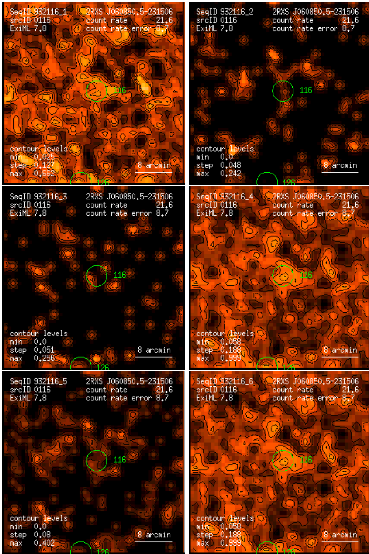
Figure 116: RASS 932116: detection 0116: band rate images, Gaussian filter: (1) PSPC channels 11 – 41, (2) 52 – 90, (3) 91 – 201, (4) 11 – 235, (5) 52 – 201, (6) 11 – 201. Broad band rates in counts/ks. Band rate contour levels in counts/ks/arcmin 2 .
