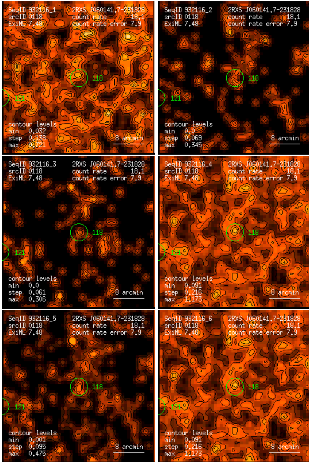
Figure 118: RASS 932116: detection 0118: band rate images, Gaussian filter: (1) PSPC channels 11 – 41, (2) 52 – 90, (3) 91 – 201, (4) 11 – 235, (5) 52 – 201, (6) 11 – 201. Broad band rates in counts/ks. Band rate contour levels in counts/ks/arcmin 2 .
