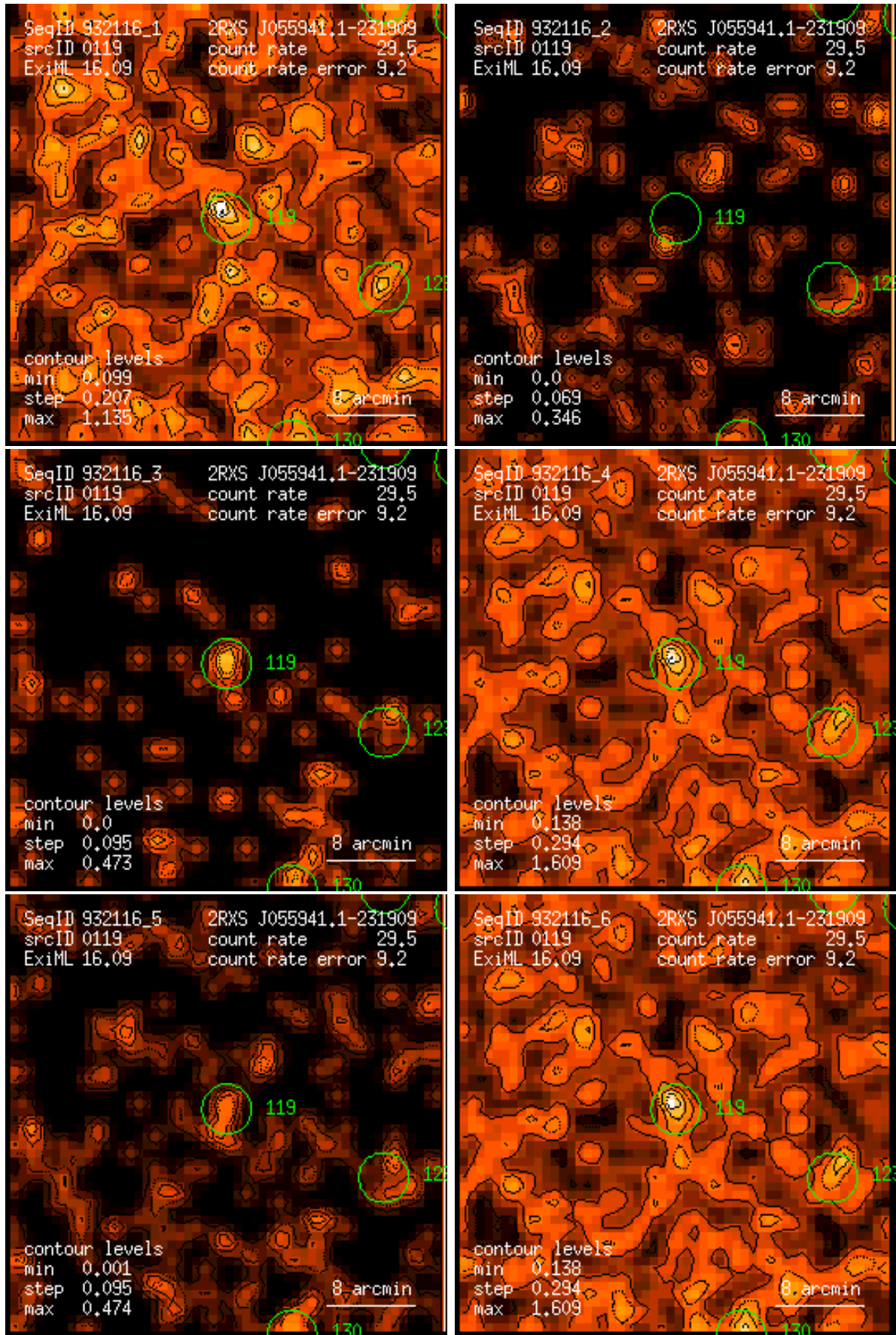
Figure 119: RASS 932116: detection 0119: band rate images, Gaussian filter: (1) PSPPC channels 11 – 41, (2) 52 – 90, (3) 91 – 201, (4) 11 – 235, (5) 52 – 201, (6) 11 – 201. Broad band rates in counts/ks. Band rate contour levels in counts/ks/arcmin 2 .
