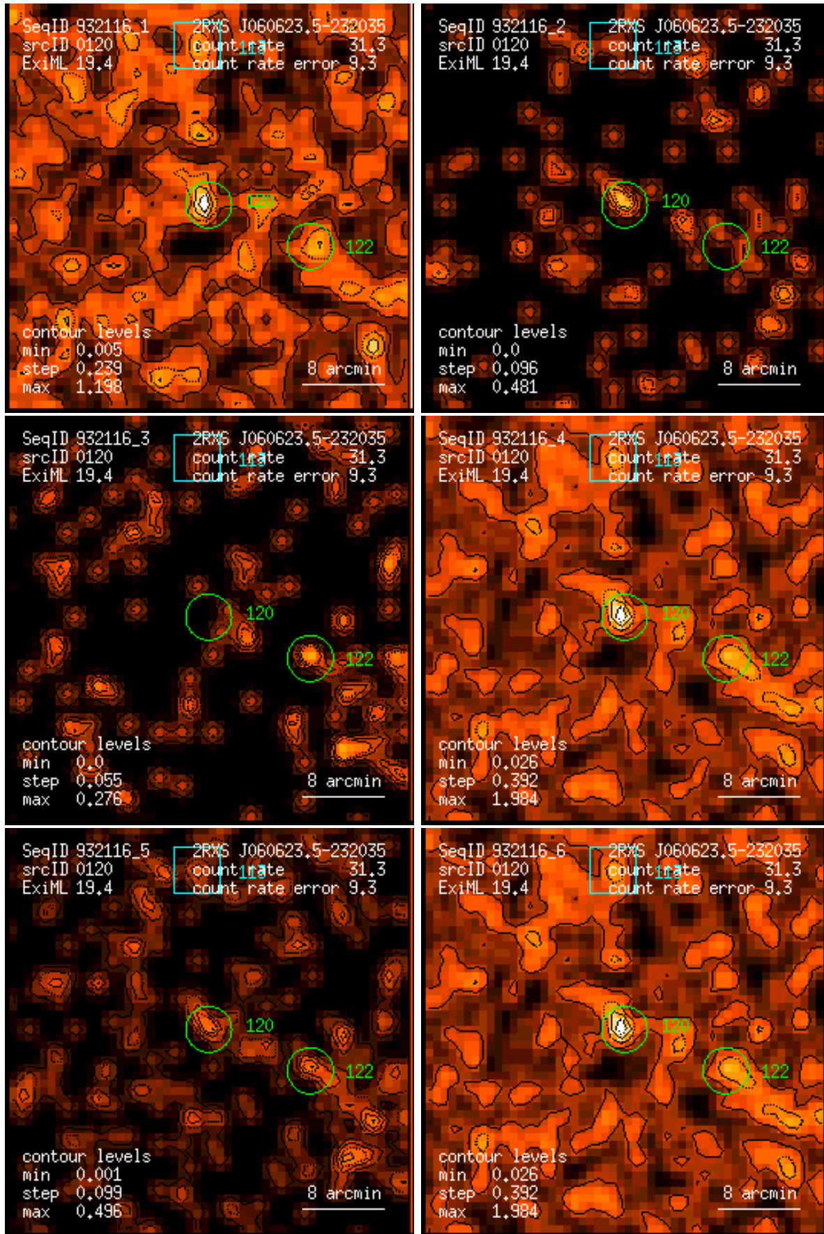
Figure 120: RASS 932116: detection 0120: band rate images, Gaussian filter: (1) PSPC channels 11 – 41, (2) 52 – 90, (3) 91 – 201, (4) 11 – 235, (5) 52 – 201, (6) 11 – 201. Broad band rates in counts/ks. Band rate contour levels in counts/ks/arcmin 2 .
