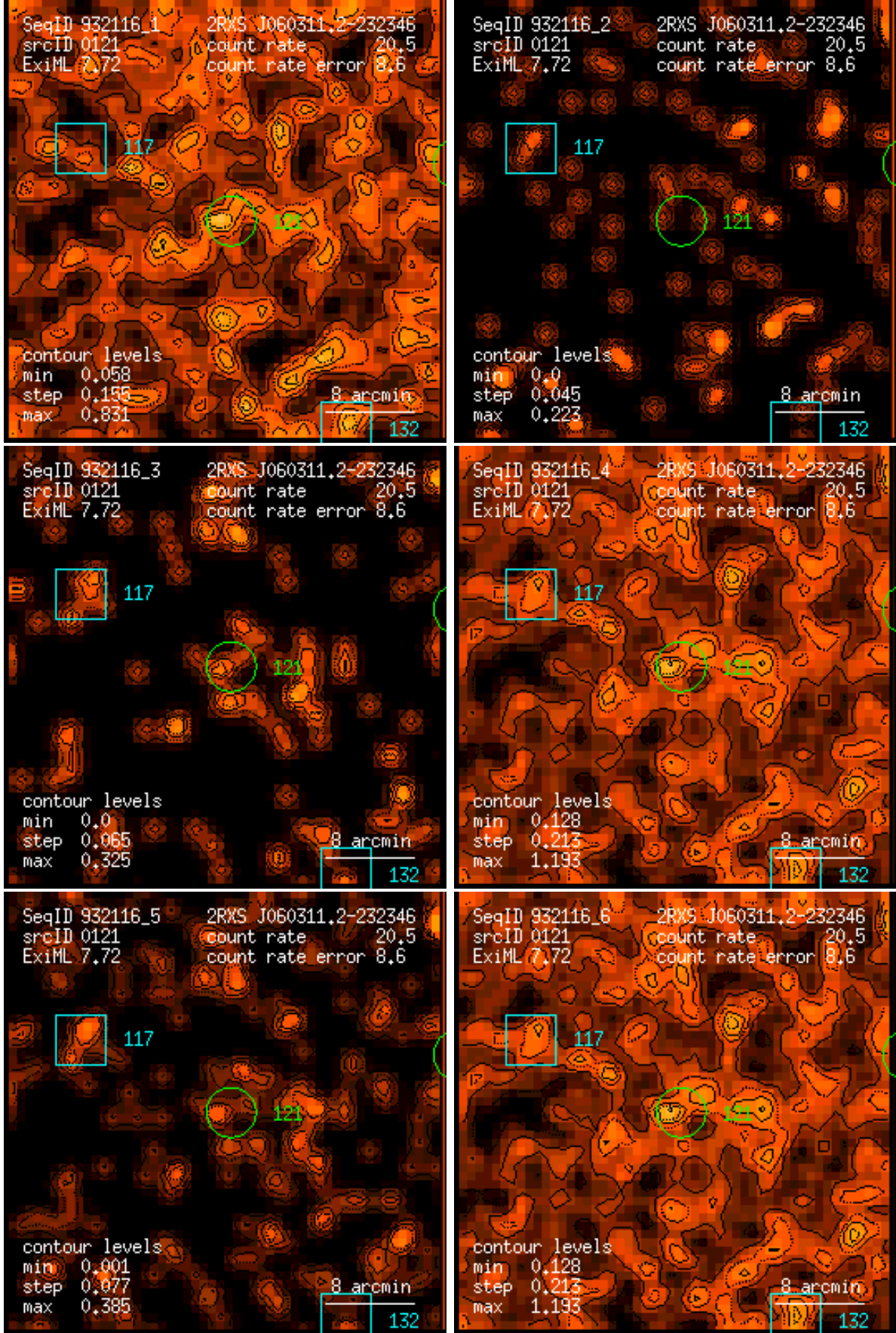
Figure 121: RASS 932116: detection 0121: band rate images, Gaussian filter: (1) PSPC channels 11 – 41, (2) 52 – 90, (3) 91 – 201, (4) 11 – 235, (5) 52 – 201, (6) 11 – 201. Broad band rates in counts/ks. Band rate contour levels in counts/ks/arcmin 2 .
