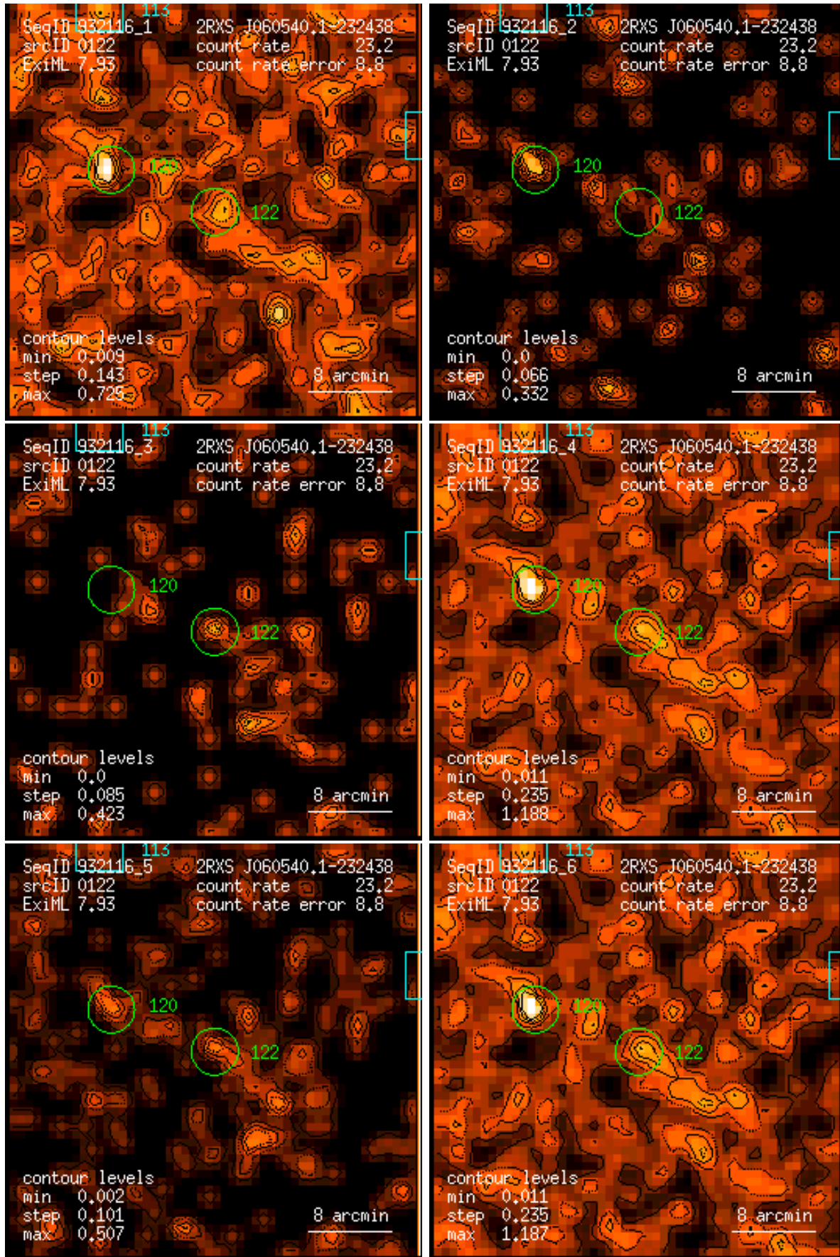
Figure 122: RASS 932116: detection 0122: band rate images, Gaussian filter: (1) PSPC channels 11 – 41, (2) 52 – 90, (3) 91 – 201, (4) 11 – 235, (5) 52 – 201, (6) 11 – 201. Broad band rates in counts/ks. Band rate contour levels in counts/ks/arcmin 2 .
