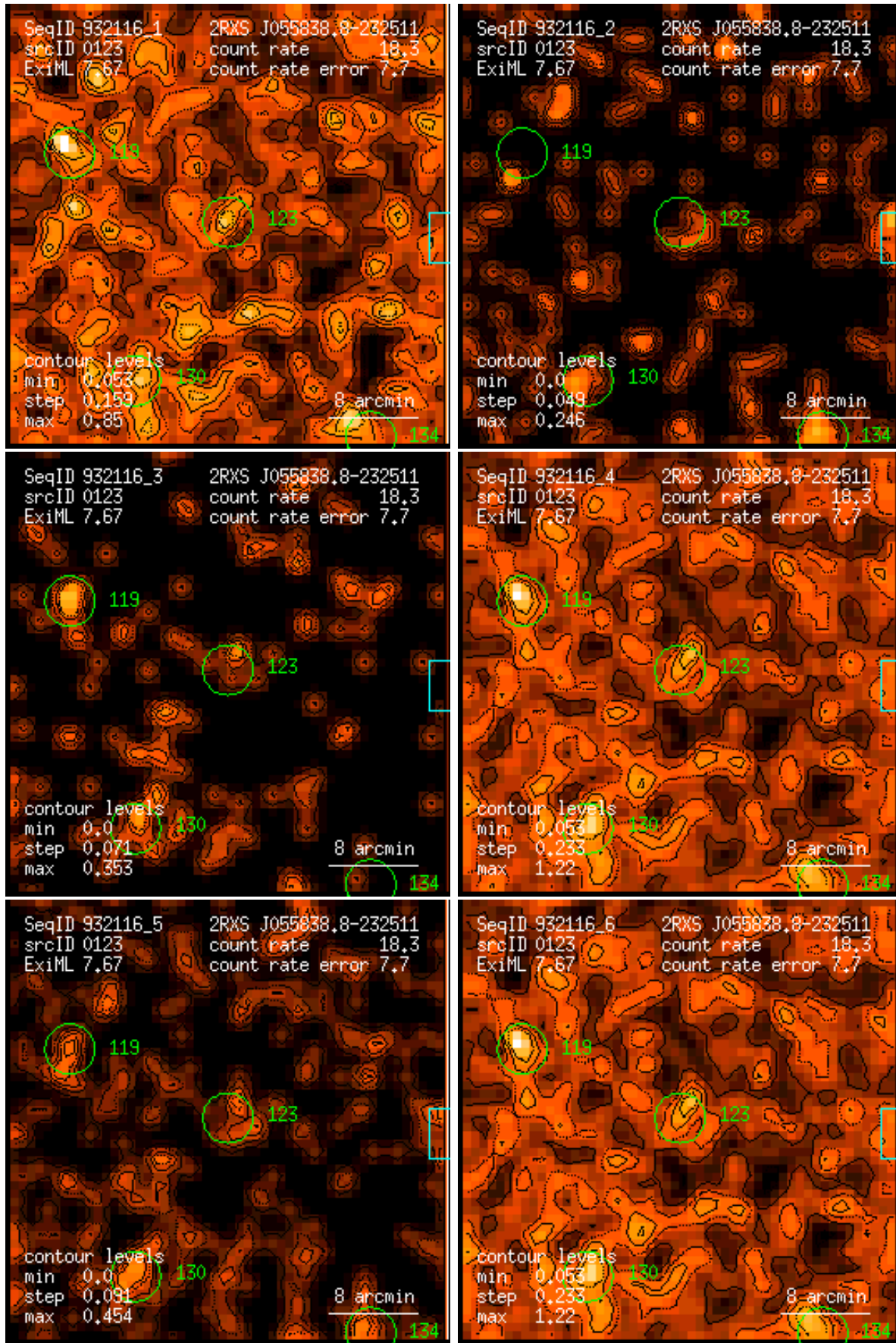
Figure 123: RASS 932116: detection 0123: band rate images, Gaussian filter: (1) PSPC channels 11 – 41, (2) 52 – 90, (3) 91 – 201, (4) 11 – 235, (5) 52 – 201, (6) 11 – 201. Broad band rates in counts/ks. Band rate contour levels in counts/ks/arcmin 2 .
