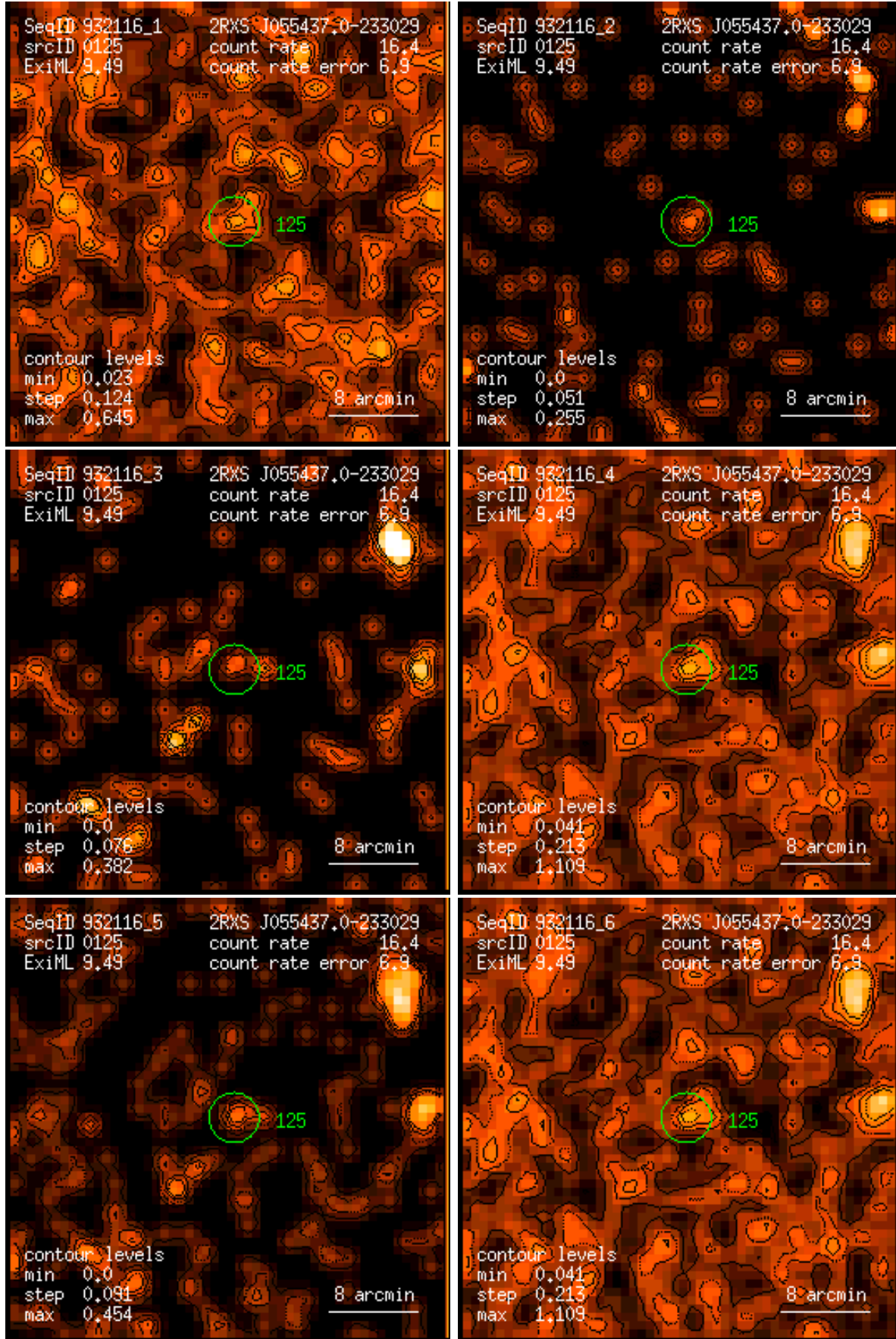
Figure 125: RASS 932116: detection 0125: band rate images, Gaussian filter: (1) PSPC channels 11 – 41, (2) 52 – 90, (3) 91 – 201, (4) 11 – 235, (5) 52 – 201, (6) 11 – 201. Broad band rates in counts/ks. Band rate contour levels in counts/ks/arcmin 2 .
