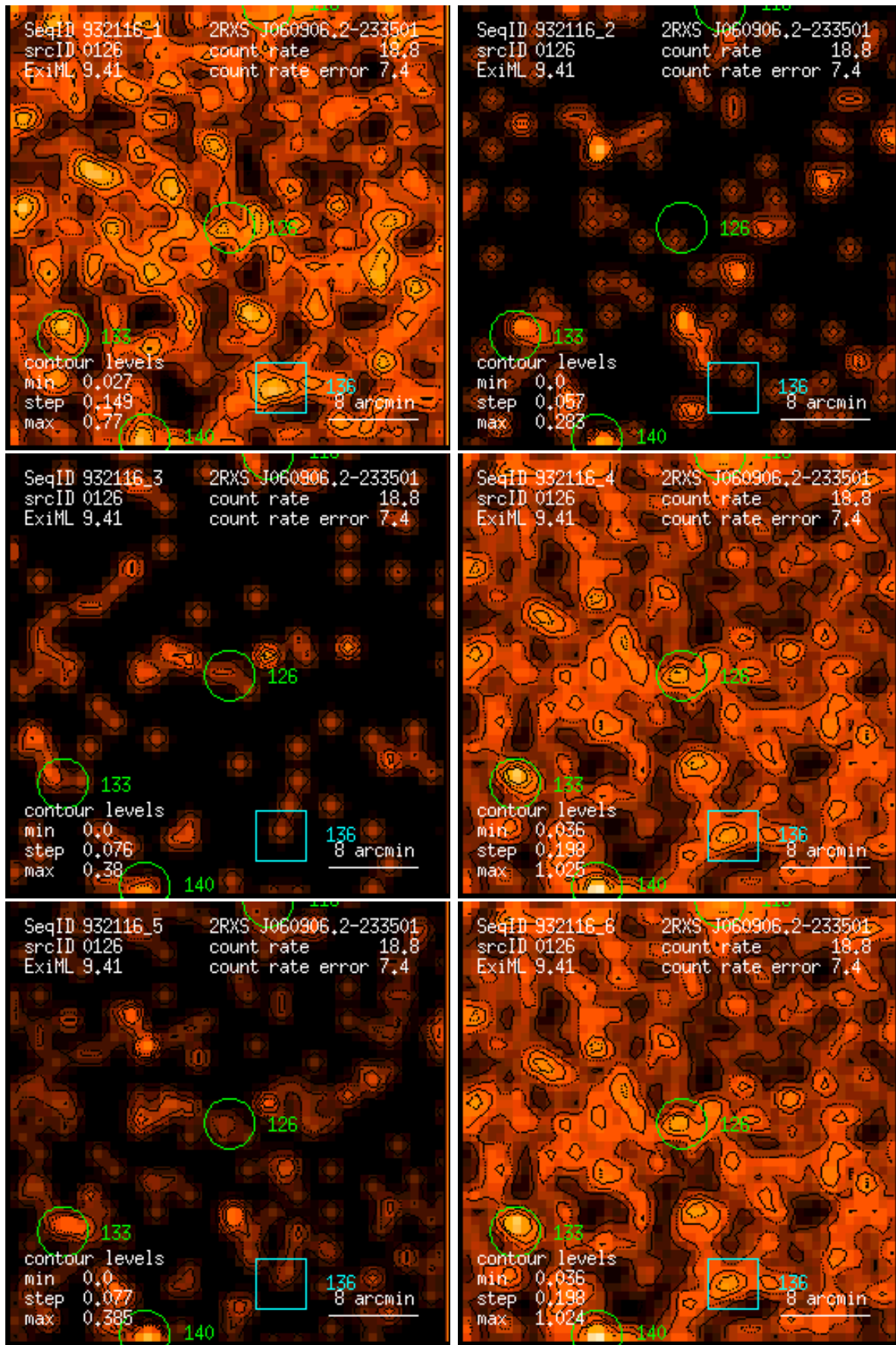
Figure 126: RASS 932116: detection 0126: band rate images, Gaussian filter: (1) PSPC channels 11 – 41, (2) 52 – 90, (3) 91 – 201, (4) 11 – 235, (5) 52 – 201, (6) 11 – 201. Broad band rates in counts/ks. Band rate contour levels in counts/ks/arcmin 2 .
