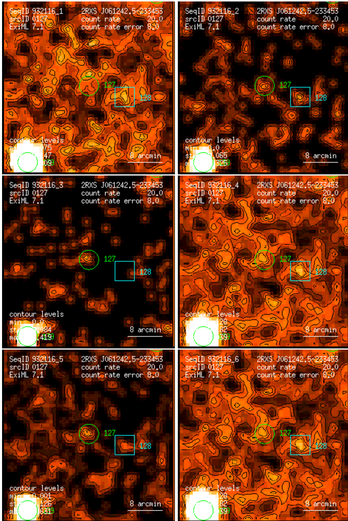
Figure 127: RASS 932116: detection 0127: band rate images, Gaussian filter: (1) PSPC channels 11 – 41, (2) 52 – 90, (3) 91 – 201, (4) 11 – 235, (5) 52 – 201, (6) 11 – 201. Broad band rates in counts/ks. Band rate contour levels in counts/ks/arcmin 2 .
