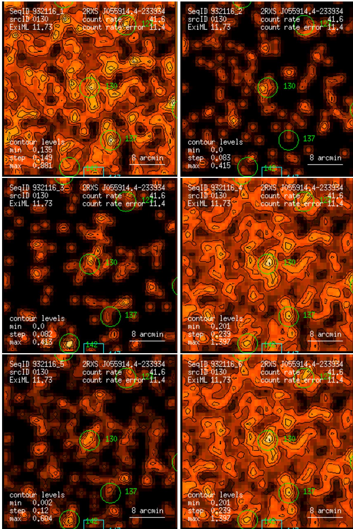
Figure 130: RASS 932116: detection 0130: band rate images, Gaussian filter: (1) PSPC channels 11 – 41, (2) 52 – 90, (3) 91 – 201, (4) 11 – 235, (5) 52 – 201, (6) 11 – 201. Broad band rates in counts/ks. Band rate contour levels in counts/ks/arcmin 2 .
