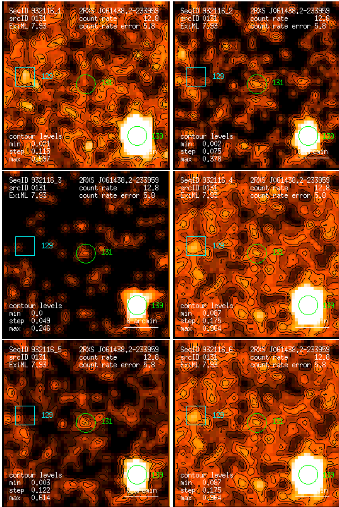
Figure 131: RASS 932116: detection 0131: band rate images, Gaussian filter: (1) PSPC channels 11 – 41, (2) 52 – 90, (3) 91 – 201, (4) 11 – 235, (5) 52 – 201, (6) 11 – 201. Broad band rates in counts/ks. Band rate contour levels in counts/ks/arcmin 2 .
