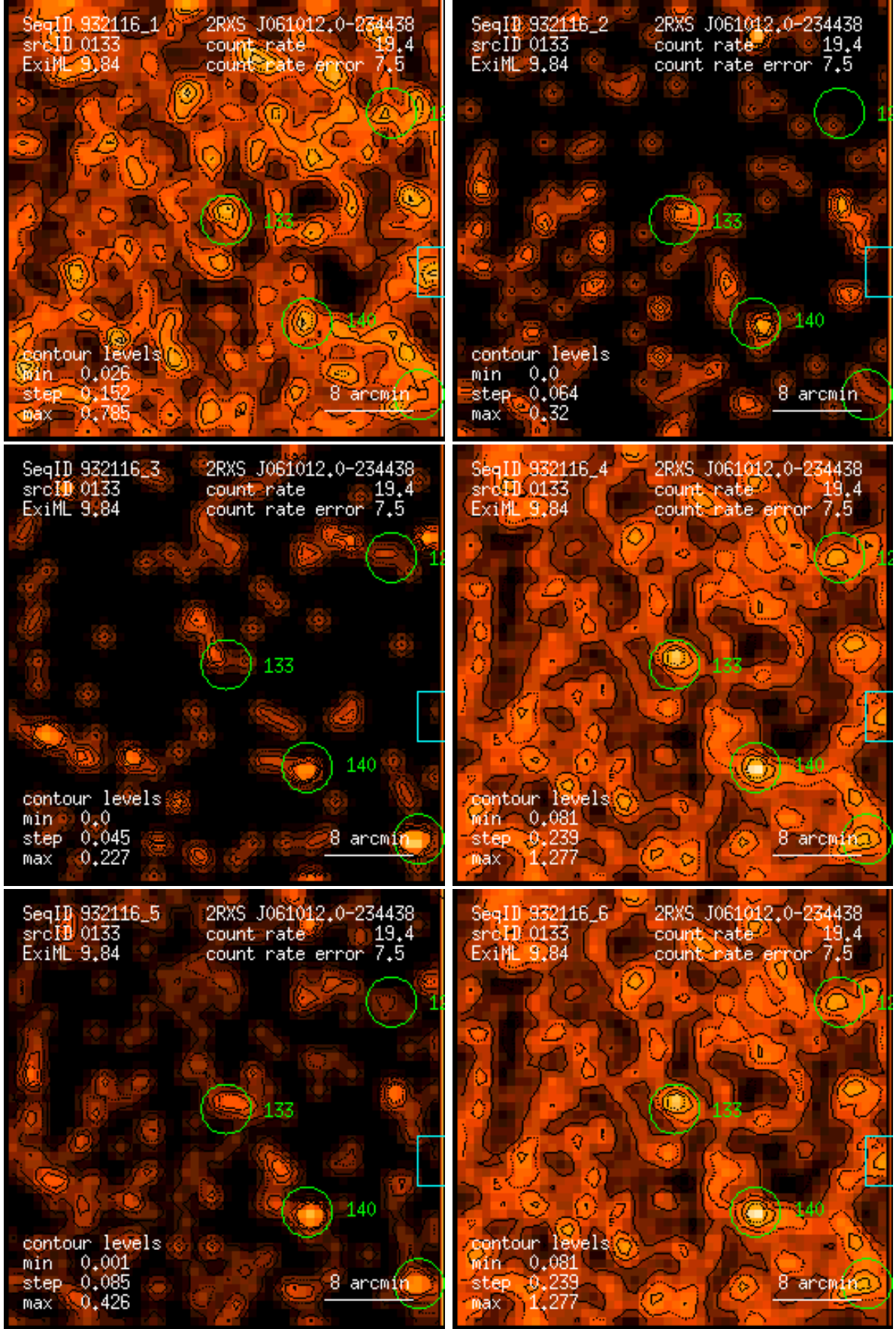
Figure 133: RASS 932116: detection 0133: band rate images, Gaussian filter: (1) PSPC channels 11 – 41, (2) 52 – 90, (3) 91 – 201, (4) 11 – 235, (5) 52 – 201, (6) 11 – 201. Broad band rates in counts/ks. Band rate contour levels in counts/ks/arcmin 2 .
