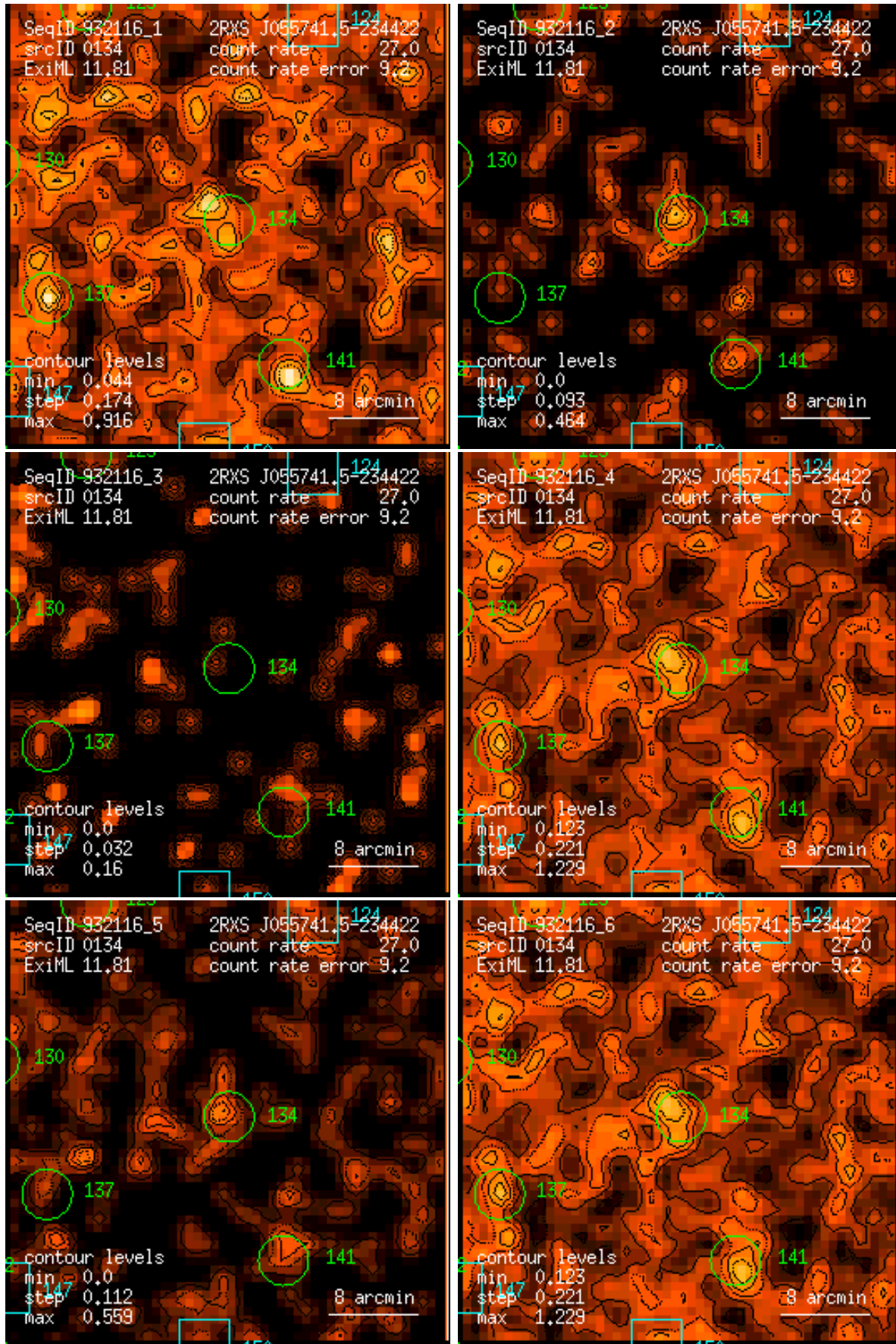
Figure 134: RASS 932116: detection 0134: band rate images, Gaussian filter: (1) PSPC channels 11 – 41, (2) 52 – 90, (3) 91 – 201, (4) 11 – 235, (5) 52 – 201, (6) 11 – 201. Broad band rates in counts/ks. Band rate contour levels in counts/ks/arcmin 2 .
