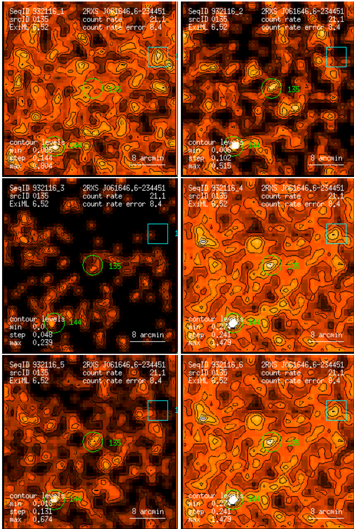
Figure 135: RASS 932116: detection 0135: band rate images, Gaussian filter: (1) PSPC channels 11 – 41, (2) 52 – 90, (3) 91 – 201, (4) 11 – 235, (5) 52 – 201, (6) 11 – 201. Broad band rates in counts/ks. Band rate contour levels in counts/ks/arcmin 2 .
