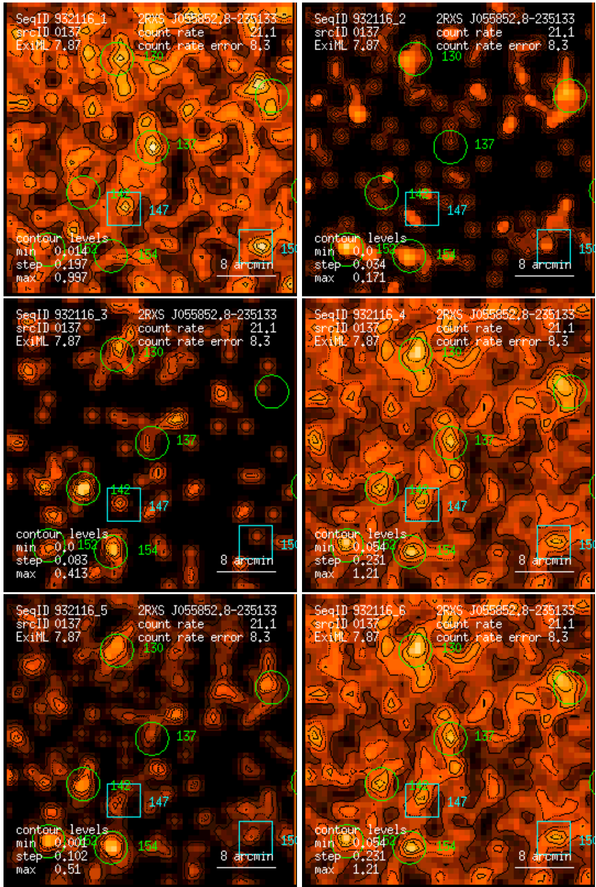
Figure 137: RASS 932116: detection 0137: band rate images, Gaussian filter: (1) PSPC channels 11 – 41, (2) 52 – 90, (3) 91 – 201, (4) 11 – 235, (5) 52 – 201, (6) 11 – 201. Broad band rates in counts/ks. Band rate contour levels in counts/ks/arcmin 2 .
