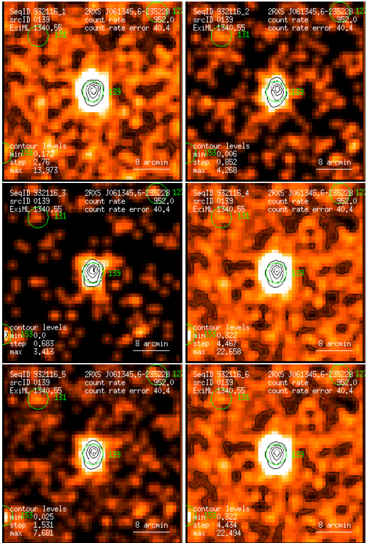
Figure 139: RASS 932116: detection 0139: band rate images, Gaussian filter: (1) PSPC channels 11 – 41, (2) 52 – 90, (3) 91 – 201, (4) 11 – 235, (5) 52 – 201, (6) 11 – 201. Broad band rates in counts/ks. Band rate contour levels in counts/ks/arcmin 2 .
