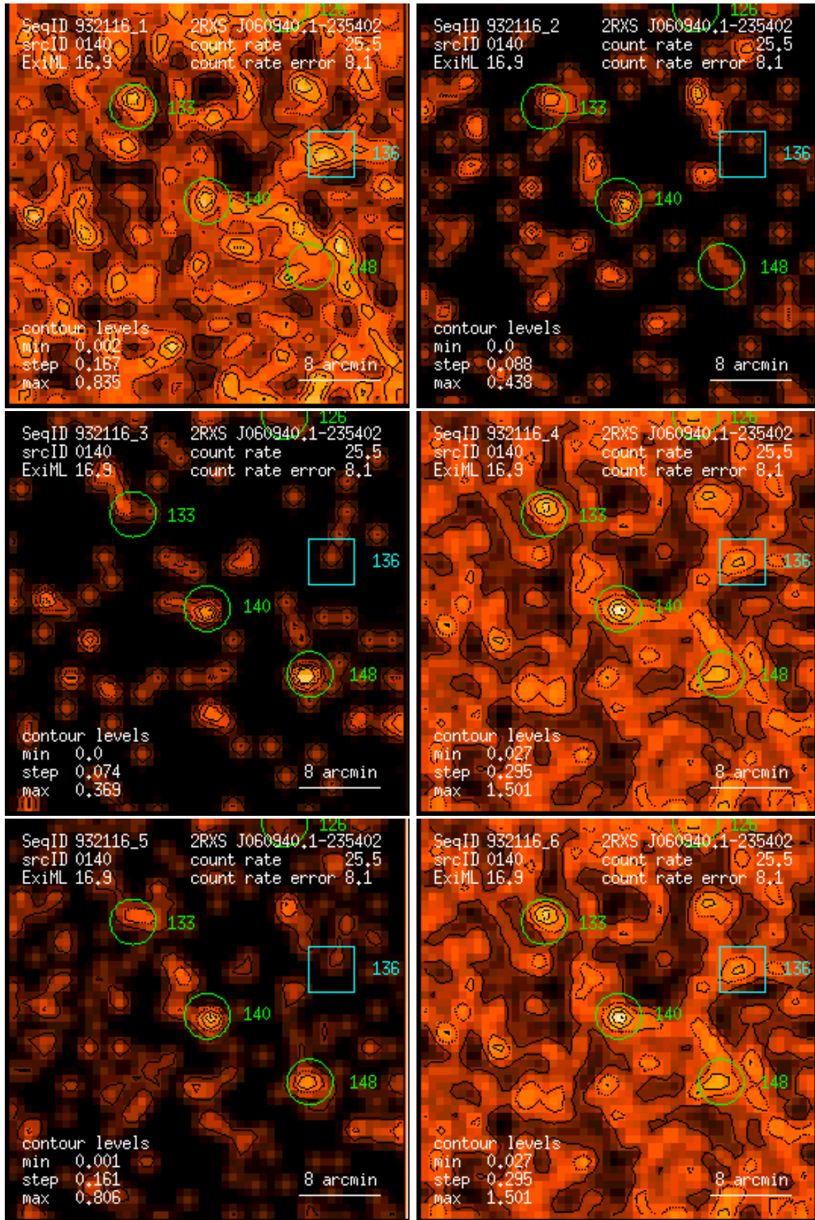
Figure 140: RASS 932116: detection 0140: band rate images, Gaussian filter: (1) PSPC channels 11 – 41, (2) 52 – 90, (3) 91 – 201, (4) 11 – 235, (5) 52 – 201, (6) 11 – 201. Broad band rates in counts/ks. Band rate contour levels in counts/ks/arcmin 2 .
