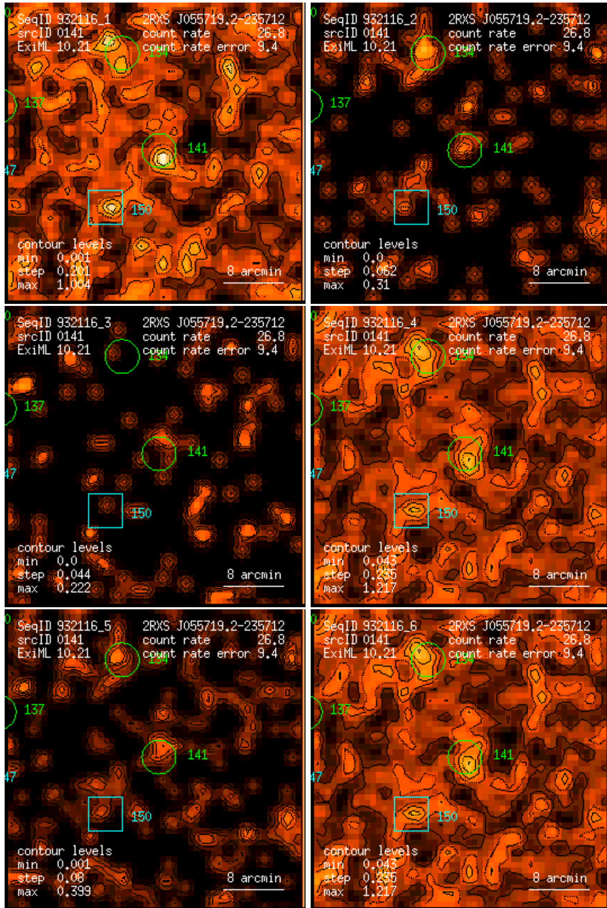
Figure 141: RASS 932116: detection 0141: band rate images, Gaussian filter: (1) PSPC channels 11 – 41, (2) 52 – 90, (3) 91 – 201, (4) 11 – 235, (5) 52 – 201, (6) 11 – 201. Broad band rates in counts/ks. Band rate contour levels in counts/ks/arcmin 2 .
