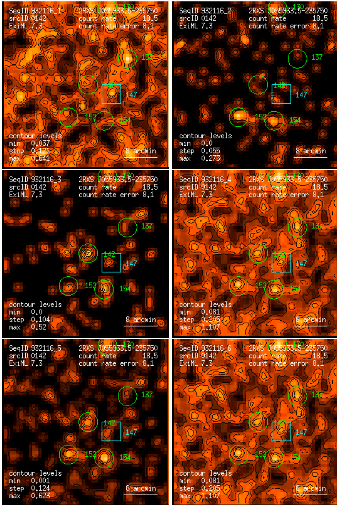
Figure 142: RASS 932116: detection 0142: band rate images, Gaussian filter: (1) PSPC channels 11 – 41, (2) 52 – 90, (3) 91 – 201, (4) 11 – 235, (5) 52 – 201, (6) 11 – 201. Broad band rates in counts/ks. Band rate contour levels in counts/ks/arcmin 2 .
