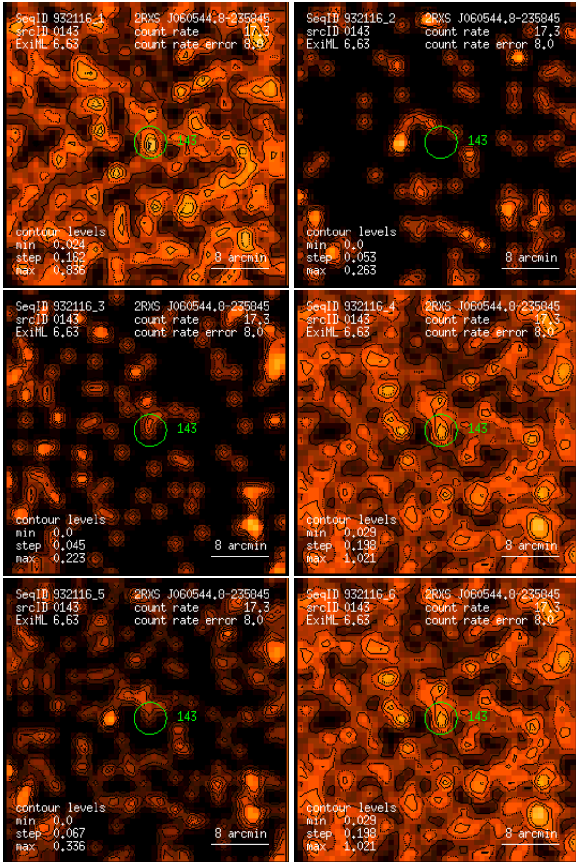
Figure 143: RASS 932116: detection 0143: band rate images, Gaussian filter: (1) PSPC channels 11 – 41, (2) 52 – 90, (3) 91 – 201, (4) 11 – 235, (5) 52 – 201, (6) 11 – 201. Broad band rates in counts/ks. Band rate contour levels in counts/ks/arcmin 2 .
