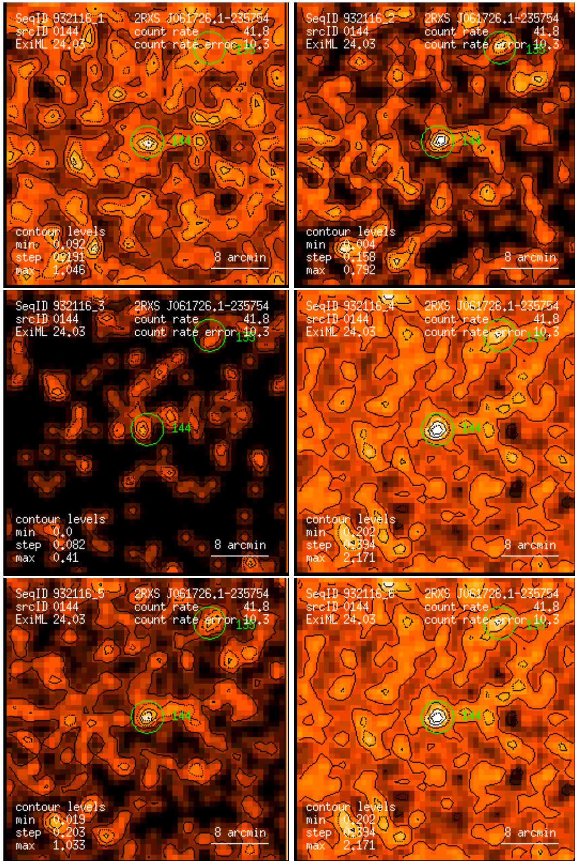
Figure 144: RASS 932116: detection 0144: band rate images, Gaussian filter: (1) PSPC channels 11 – 41, (2) 52 – 90, (3) 91 – 201, (4) 11 – 235, (5) 52 – 201, (6) 11 – 201. Broad band rates in counts/ks. Band rate contour levels in counts/ks/arcmin 2 .
