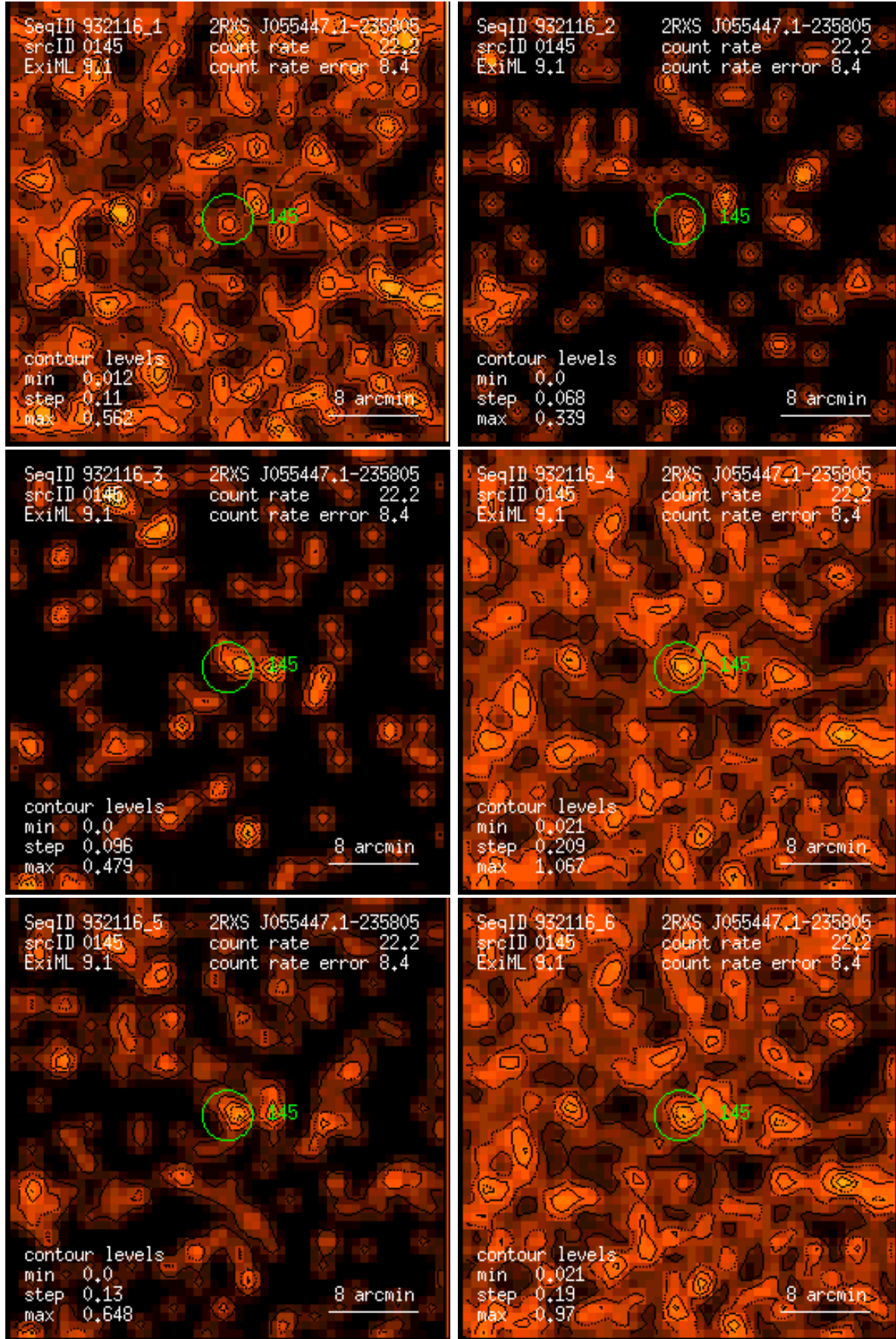
Figure 145: RASS 932116: detection 0145: band rate images, Gaussian filter: (1) PSPC channels 11 – 41, (2) 52 – 90, (3) 91 – 201, (4) 11 – 235, (5) 52 – 201, (6) 11 – 201. Broad band rates in counts/ks. Band rate contour levels in counts/ks/arcmin 2 .
