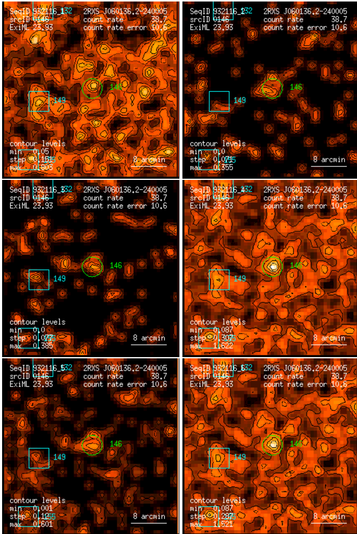
Figure 146: RASS 932116: detection 0146: band rate images, Gaussian filter: (1) PSPC channels 11 – 41, (2) 52 – 90, (3) 91 – 201, (4) 11 – 235, (5) 52 – 201, (6) 11 – 201. Broad band rates in counts/ks. Band rate contour levels in counts/ks/arcmin 2 .
