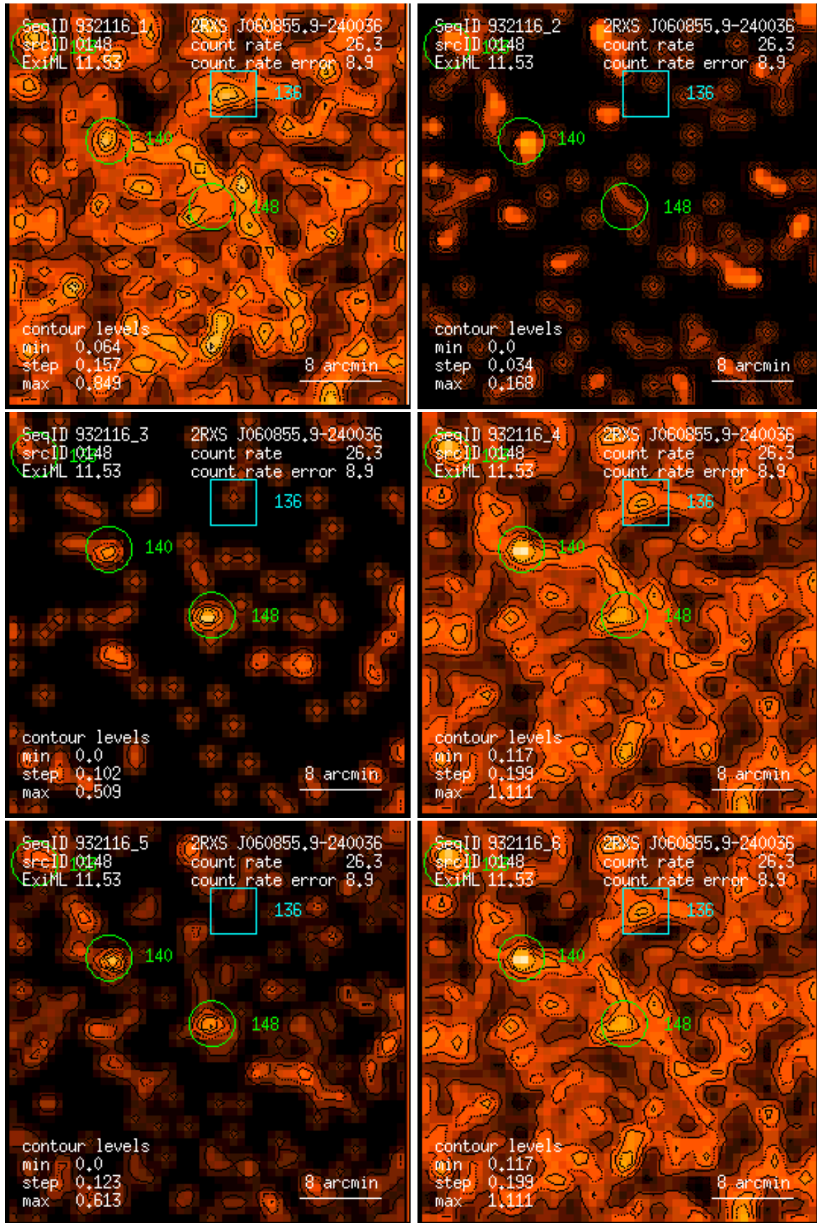
Figure 148: RASS 932116: detection 0148: band rate images, Gaussian filter: (1) PSPC channels 11 – 41, (2) 52 – 90, (3) 91 – 201, (4) 11 – 235, (5) 52 – 201, (6) 11 – 201. Broad band rates in counts/ks. Band rate contour levels in counts/ks/arcmin 2 .
