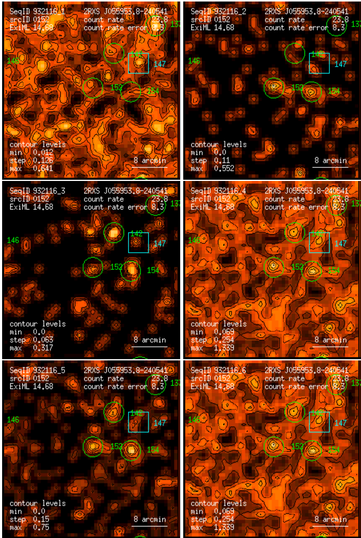
Figure 152: RASS 932116: detection 0152: band rate images, Gaussian filter: (1) PSPC channels 11 – 41, (2) 52 – 90, (3) 91 – 201, (4) 11 – 235, (5) 52 – 201, (6) 11 – 201. Broad band rates in counts/ks. Band rate contour levels in counts/ks/arcmin 2 .
