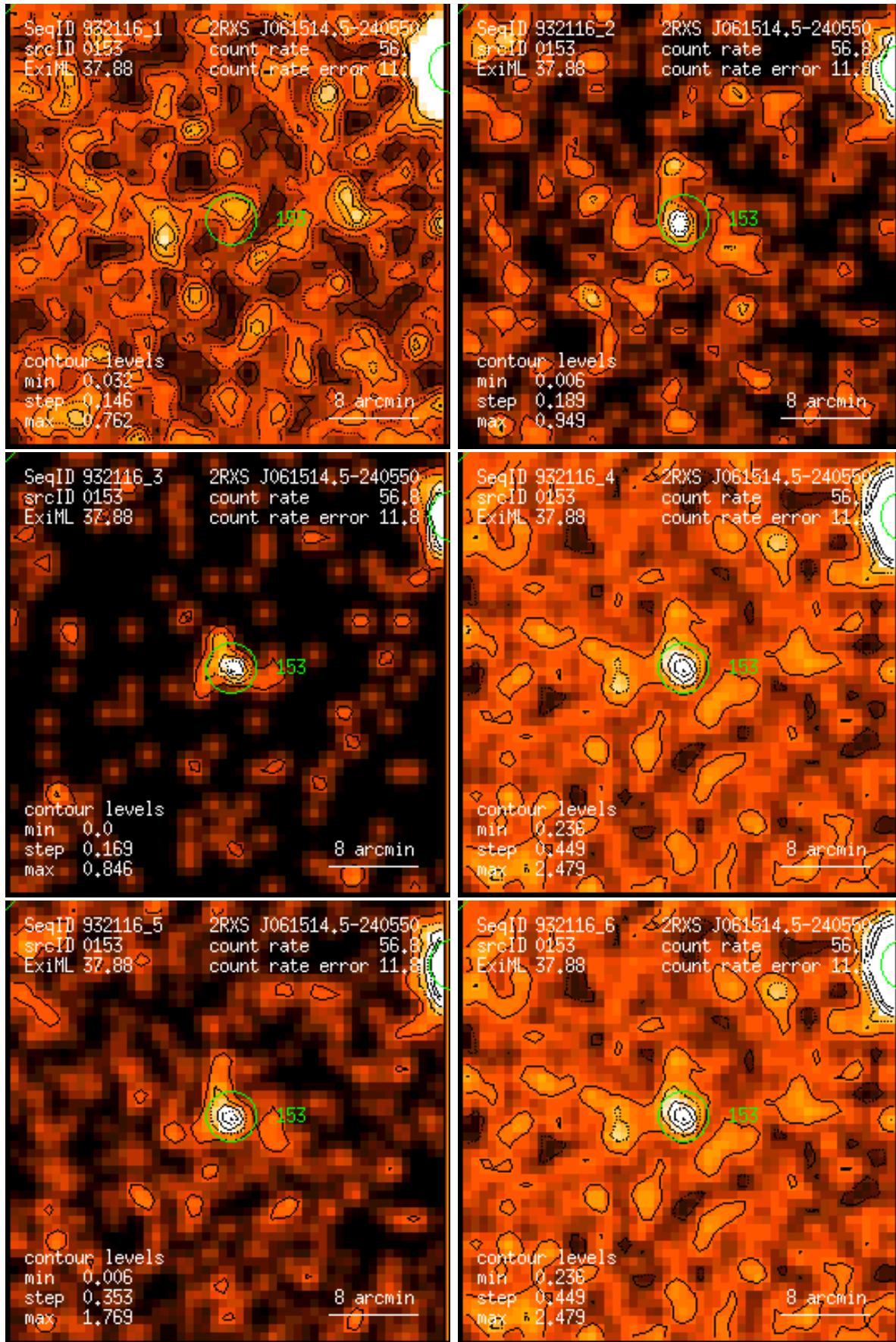
Figure 153: RASS 932116: detection 0153: band rate images, Gaussian filter: (1) PSPC channels 11 – 41, (2) 52 – 90, (3) 91 – 201, (4) 11 – 235, (5) 52 – 201, (6) 11 – 201. Broad band rates in counts/ks. Band rate contour levels in counts/ks/arcmin 2 .
