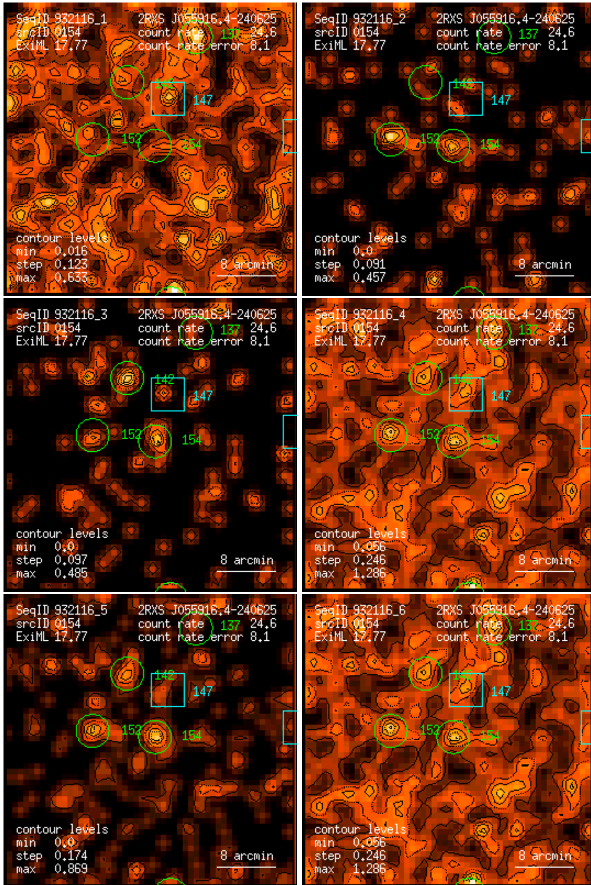
Figure 154: RASS 932116: detection 0154: band rate images, Gaussian filter: (1) PSPC channels 11 – 41, (2) 52 – 90, (3) 91 – 201, (4) 11 – 235, (5) 52 – 201, (6) 11 – 201. Broad band rates in counts/ks. Band rate contour levels in counts/ks/arcmin 2 .
