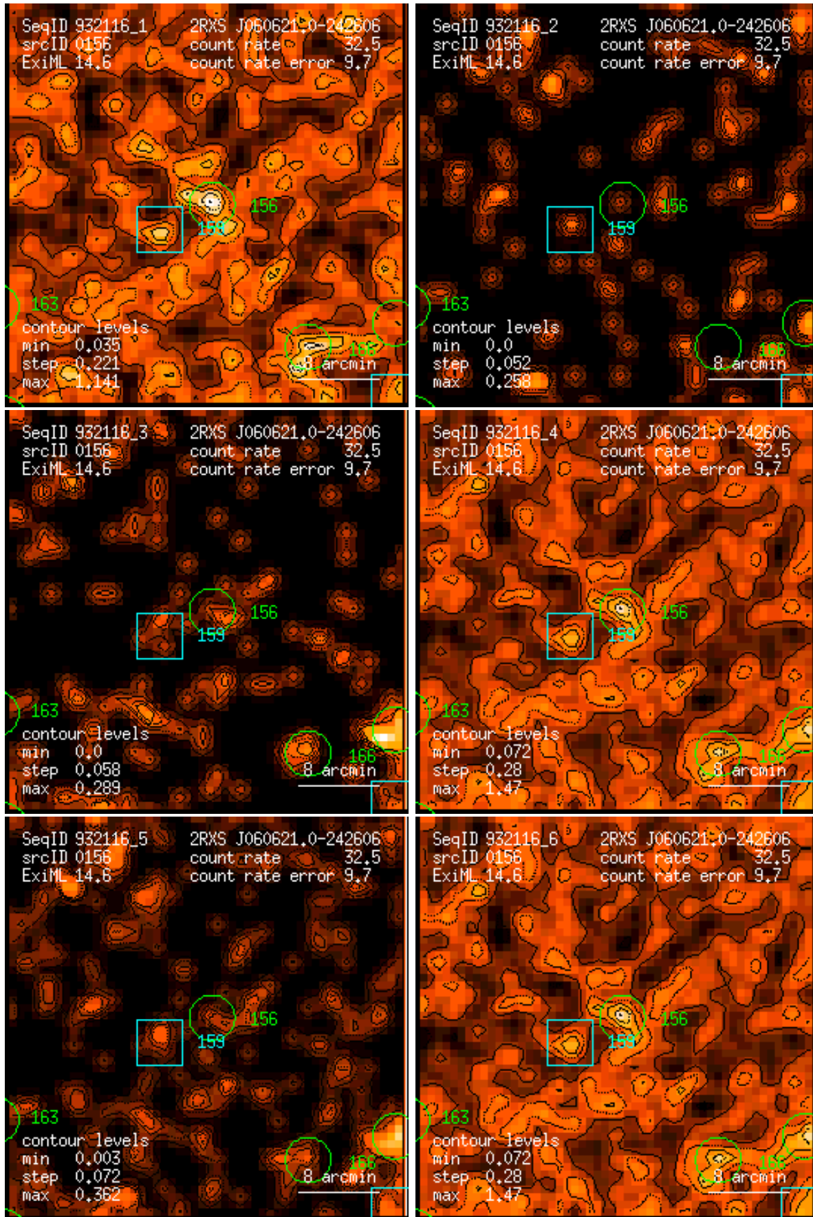
Figure 156: RASS 932116: detection 0156: band rate images, Gaussian filter: (1) PSPC channels 11 – 41, (2) 52 – 90, (3) 91 – 201, (4) 11 – 235, (5) 52 – 201, (6) 11 – 201. Broad band rates in counts/ks. Band rate contour levels in counts/ks/arcmin 2 .
