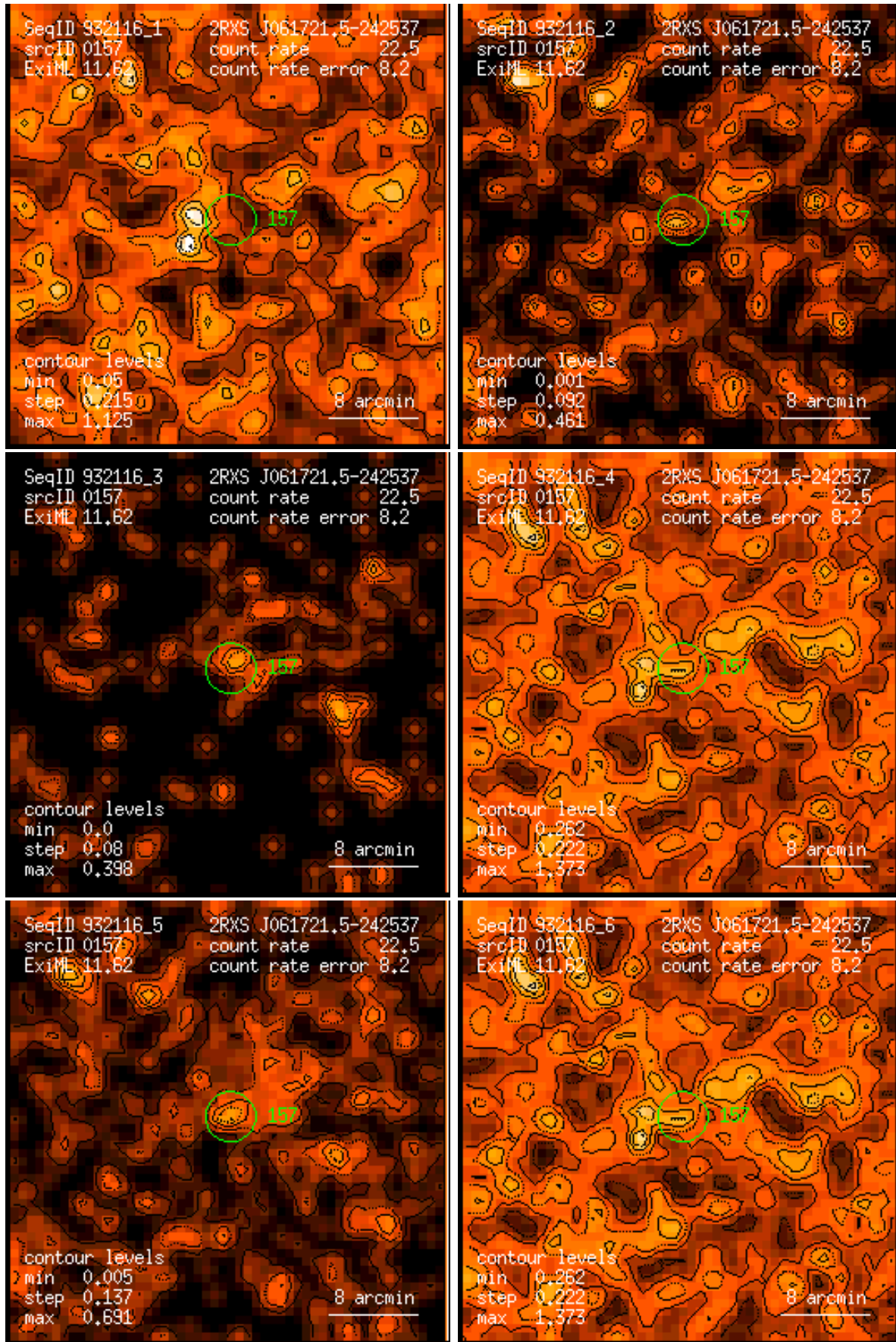
Figure 157: RASS 932116: detection 0157: band rate images, Gaussian filter: (1) PSPC channels 11 – 41, (2) 52 – 90, (3) 91 – 201, (4) 11 – 235, (5) 52 – 201, (6) 11 – 201. Broad band rates in counts/ks. Band rate contour levels in counts/ks/arcmin 2 .
