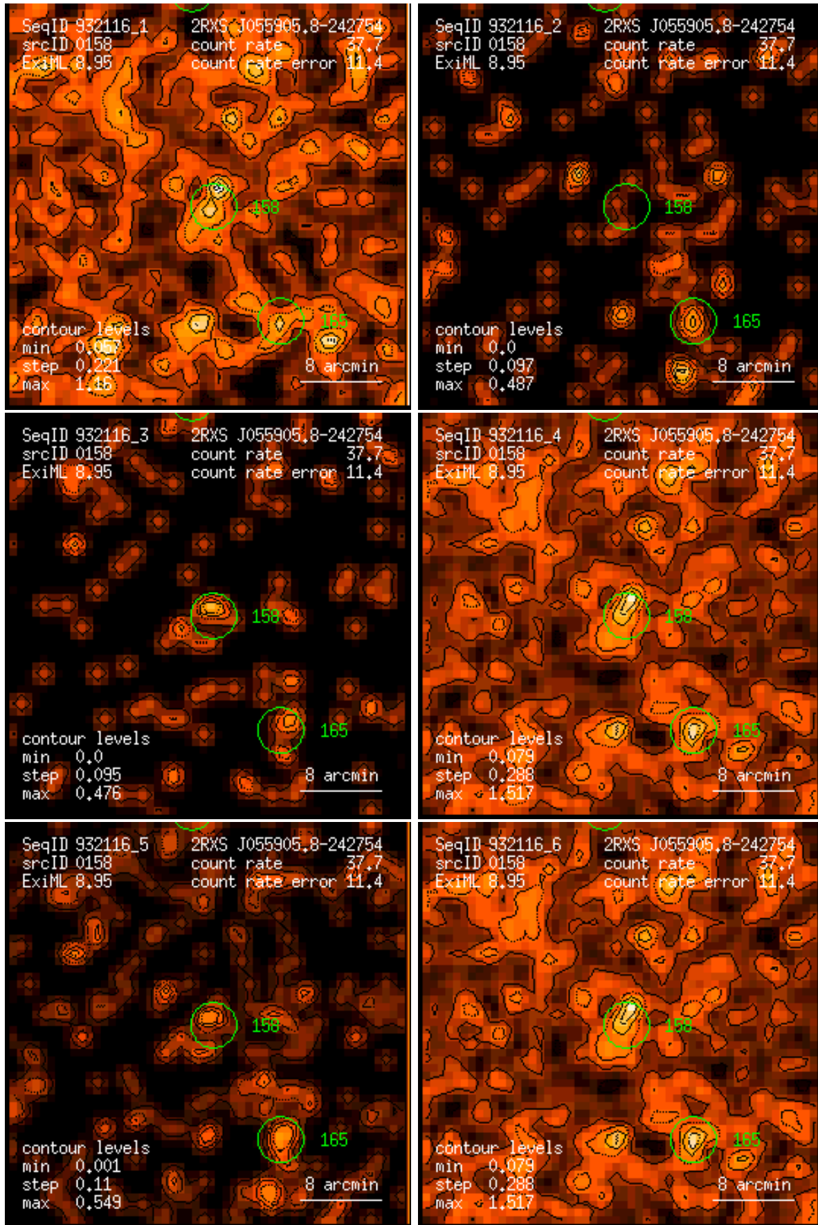
Figure 158: RASS 932116: detection 0158: band rate images, Gaussian filter: (1) PSPC channels 11 – 41, (2) 52 – 90, (3) 91 – 201, (4) 11 – 235, (5) 52 – 201, (6) 11 – 201. Broad band rates in counts/ks. Band rate contour levels in counts/ks/arcmin 2 .
