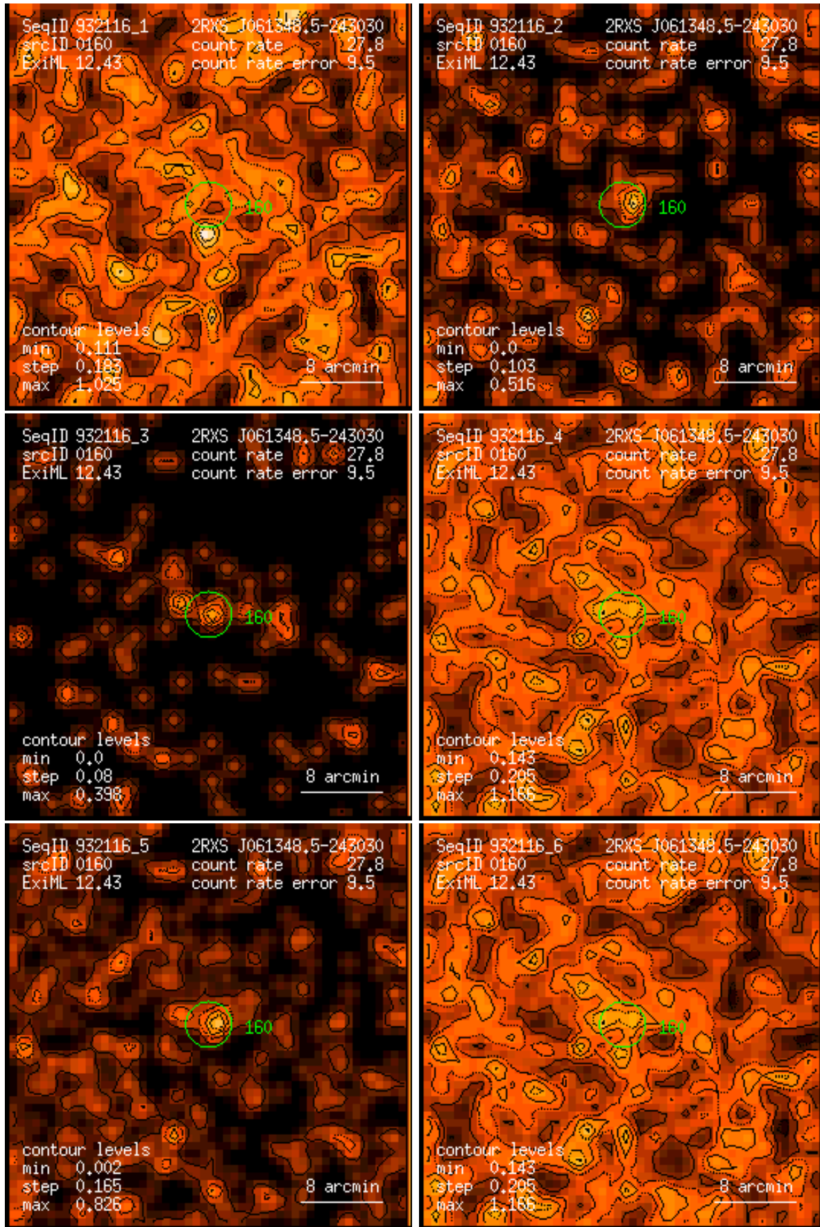
Figure 160: RASS 932116: detection 0160: band rate images, Gaussian filter: (1) PSPC channels 11 – 41, (2) 52 – 90, (3) 91 – 201, (4) 11 – 235, (5) 52 – 201, (6) 11 – 201. Broad band rates in counts/ks. Band rate contour levels in counts/ks/arcmin 2 .
