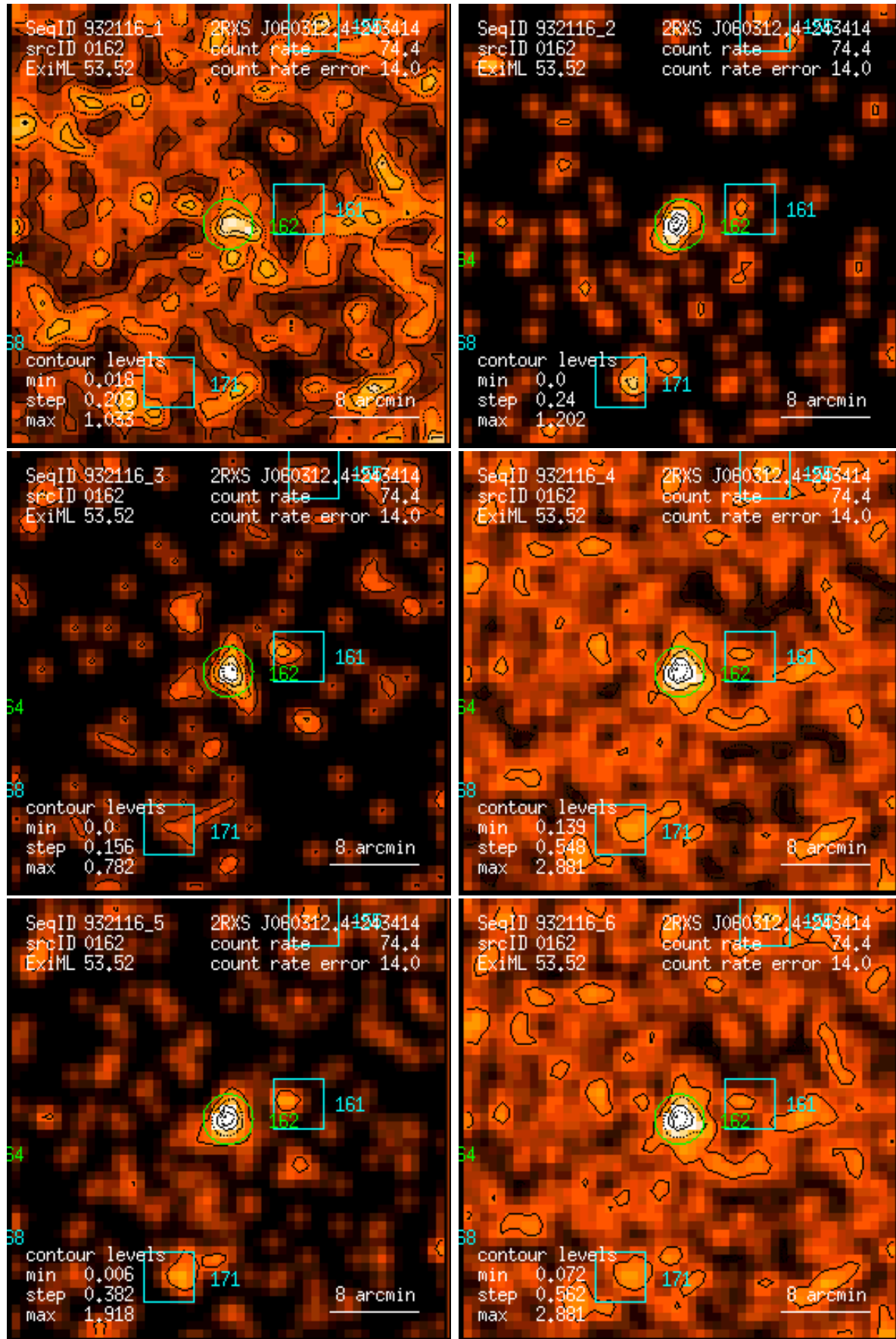
Figure 162: RASS 932116: detection 0162: band rate images, Gaussian filter: (1) PSPC channels 11 – 41, (2) 52 – 90, (3) 91 – 201, (4) 11 – 235, (5) 52 – 201, (6) 11 – 201. Broad band rates in counts/ks. Band rate contour levels in counts/ks/arcmin 2 .
