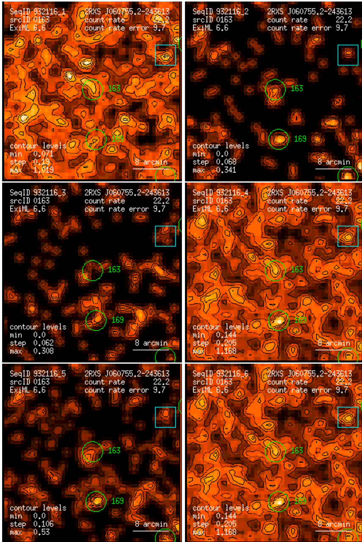
Figure 163: RASS 932116: detection 0163: band rate images, Gaussian filter: (1) PSPC channels 11 – 41, (2) 52 – 90, (3) 91 – 201, (4) 11 – 235, (5) 52 – 201, (6) 11 – 201. Broad band rates in counts/ks. Band rate contour levels in counts/ks/arcmin 2 .
