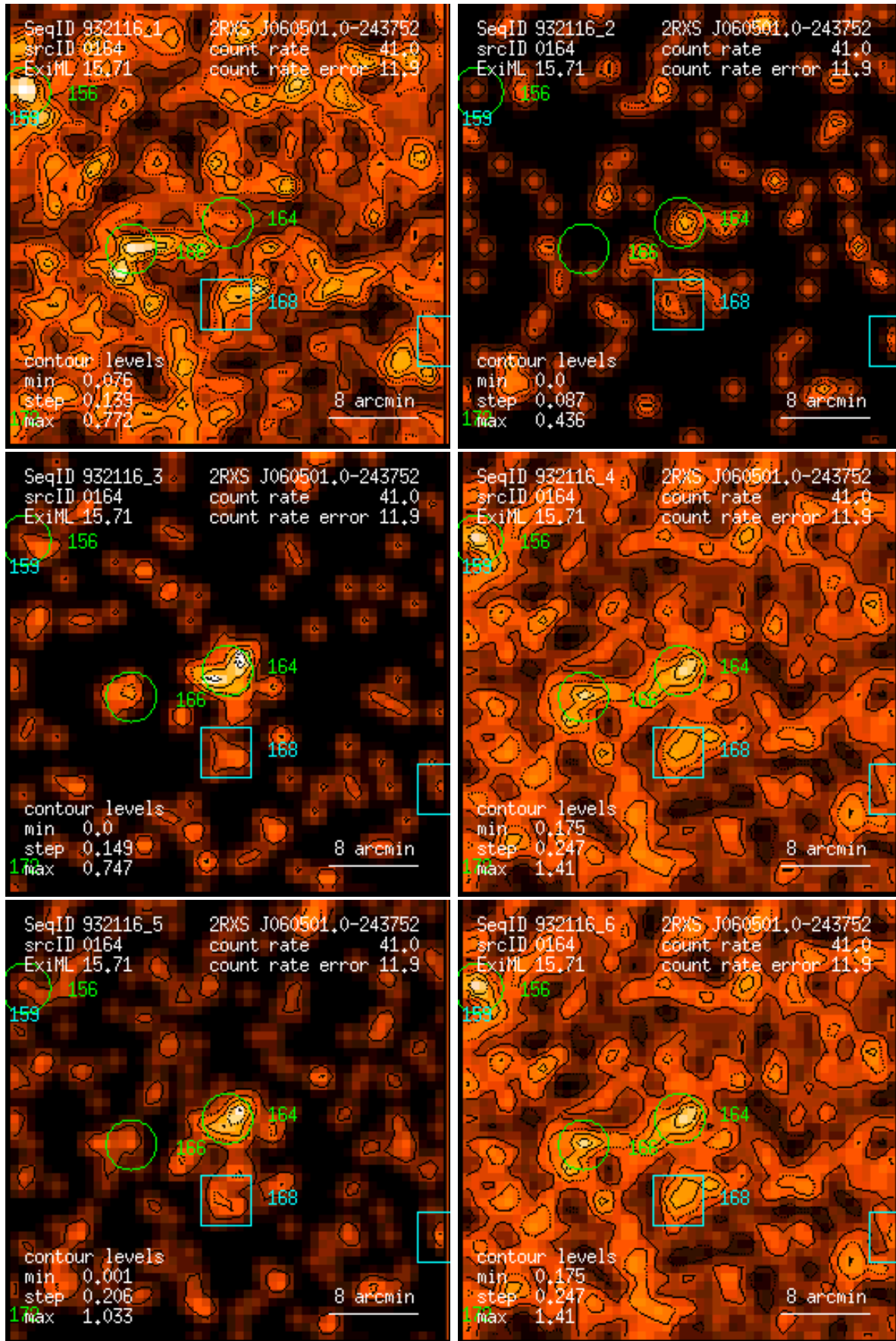
Figure 164: RASS 932116: detection 0164: band rate images, Gaussian filter: (1) PSPC channels 11 – 41, (2) 52 – 90, (3) 91 – 201, (4) 11 – 235, (5) 52 – 201, (6) 11 – 201. Broad band rates in counts/ks. Band rate contour levels in counts/ks/arcmin 2 .
